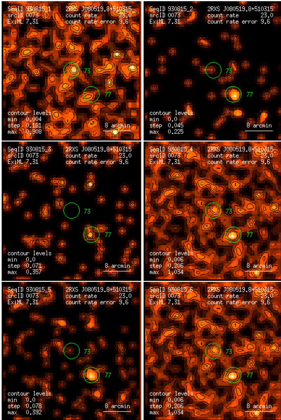
Figure 73: RASS 930815: detection 0073: band rate images, Gaussian filter: (1) PSPC channels 11 – 41, (2) 52 – 90, (3) 91 – 201, (4) 11 – 235, (5) 52 – 201, (6) 11 – 201. Broad band rates in counts/ks. Band rate contour levels in counts/ks/arcmin 2 .
