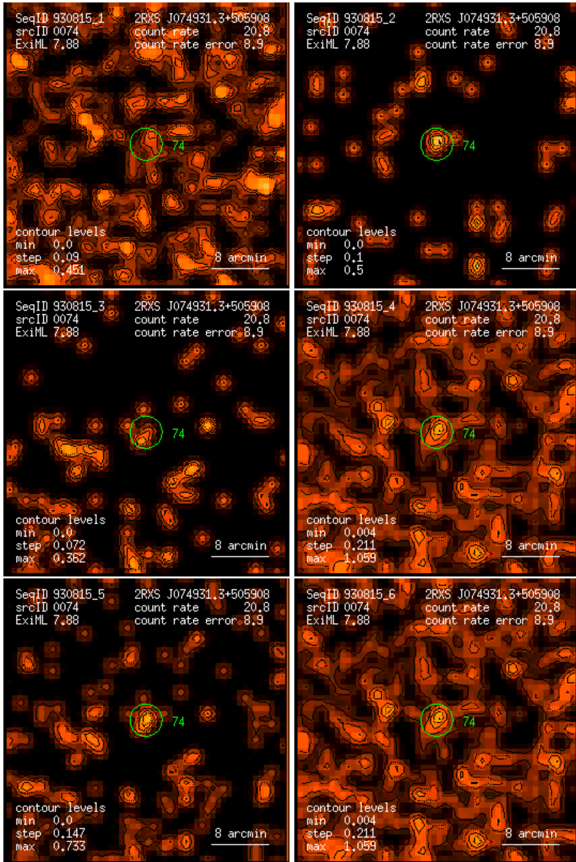
Figure 74: RASS 930815: detection 0074: band rate images, Gaussian filter: (1) PSPC channels 11 – 41, (2) 52 – 90, (3) 91 – 201, (4) 11 – 235, (5) 52 – 201, (6) 11 – 201. Broad band rates in counts/ks. Band rate contour levels in counts/ks/arcmin 2 .
