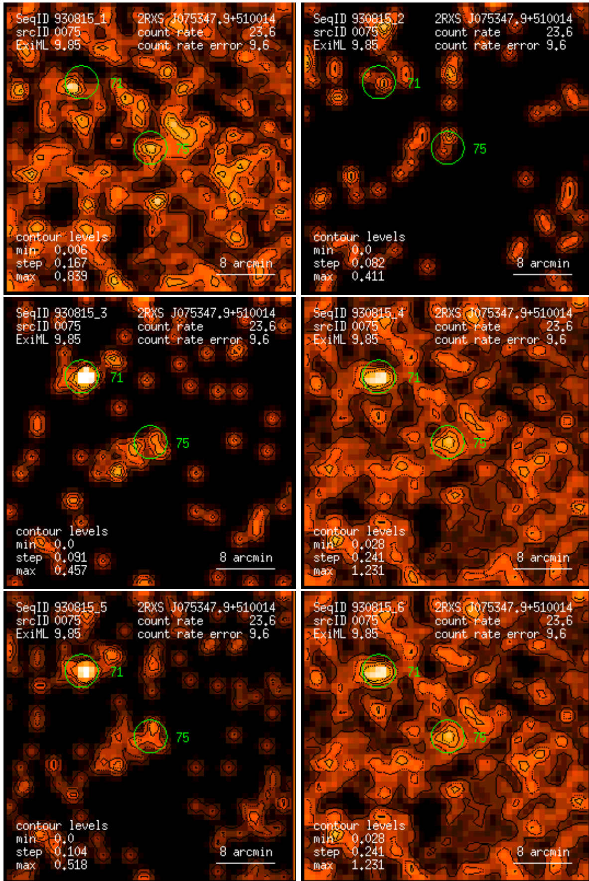
Figure 75: RASS 930815: detection 0075: band rate images, Gaussian filter: (1) PSPC channels 11 – 41, (2) 52 – 90, (3) 91 – 201, (4) 11 – 235, (5) 52 – 201, (6) 11 – 201. Broad band rates in counts/ks. Band rate contour levels in counts/ks/arcmin 2 .
