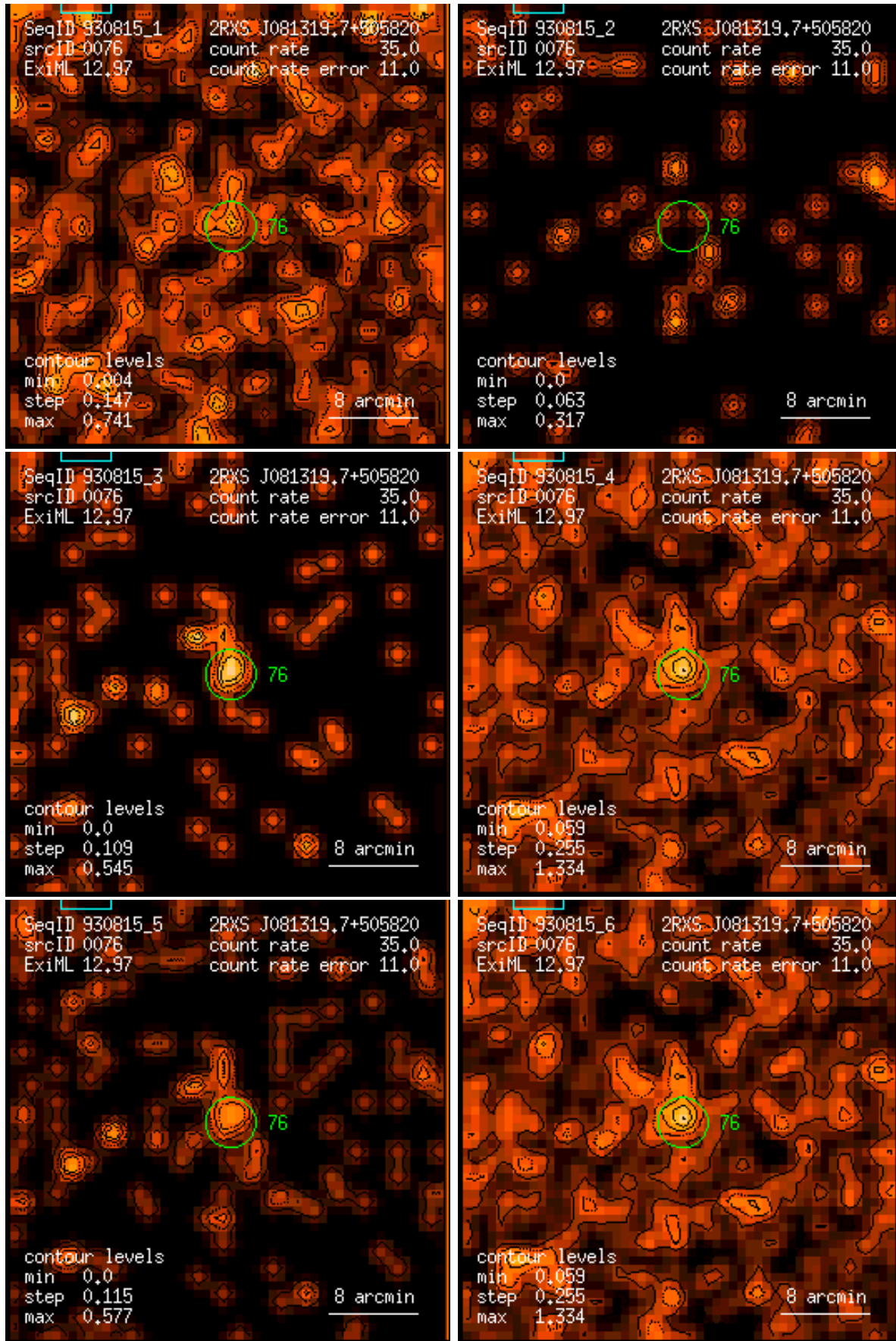
Figure 76: RASS 930815: detection 0076: band rate images, Gaussian filter: (1) PSPC channels 11 – 41, (2) 52 – 90, (3) 91 – 201, (4) 11 – 235, (5) 52 – 201, (6) 11 – 201. Broad band rates in counts/ks. Band rate contour levels in counts/ks/arcmin 2 .
