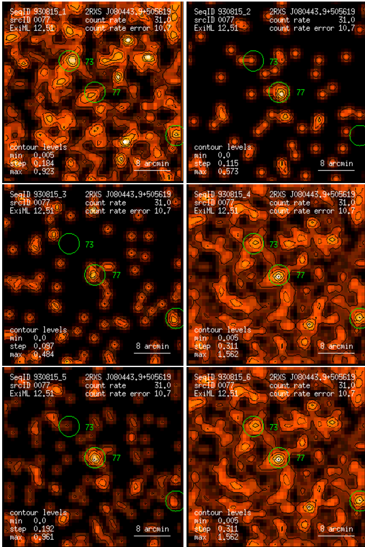
Figure 77: RASS 930815: detection 0077: band rate images, Gaussian filter: (1) PSPC channels 11 – 41, (2) 52 – 90, (3) 91 – 201, (4) 11 – 235, (5) 52 – 201, (6) 11 – 201. Broad band rates in counts/ks. Band rate contour levels in counts/ks/arcmin 2 .
