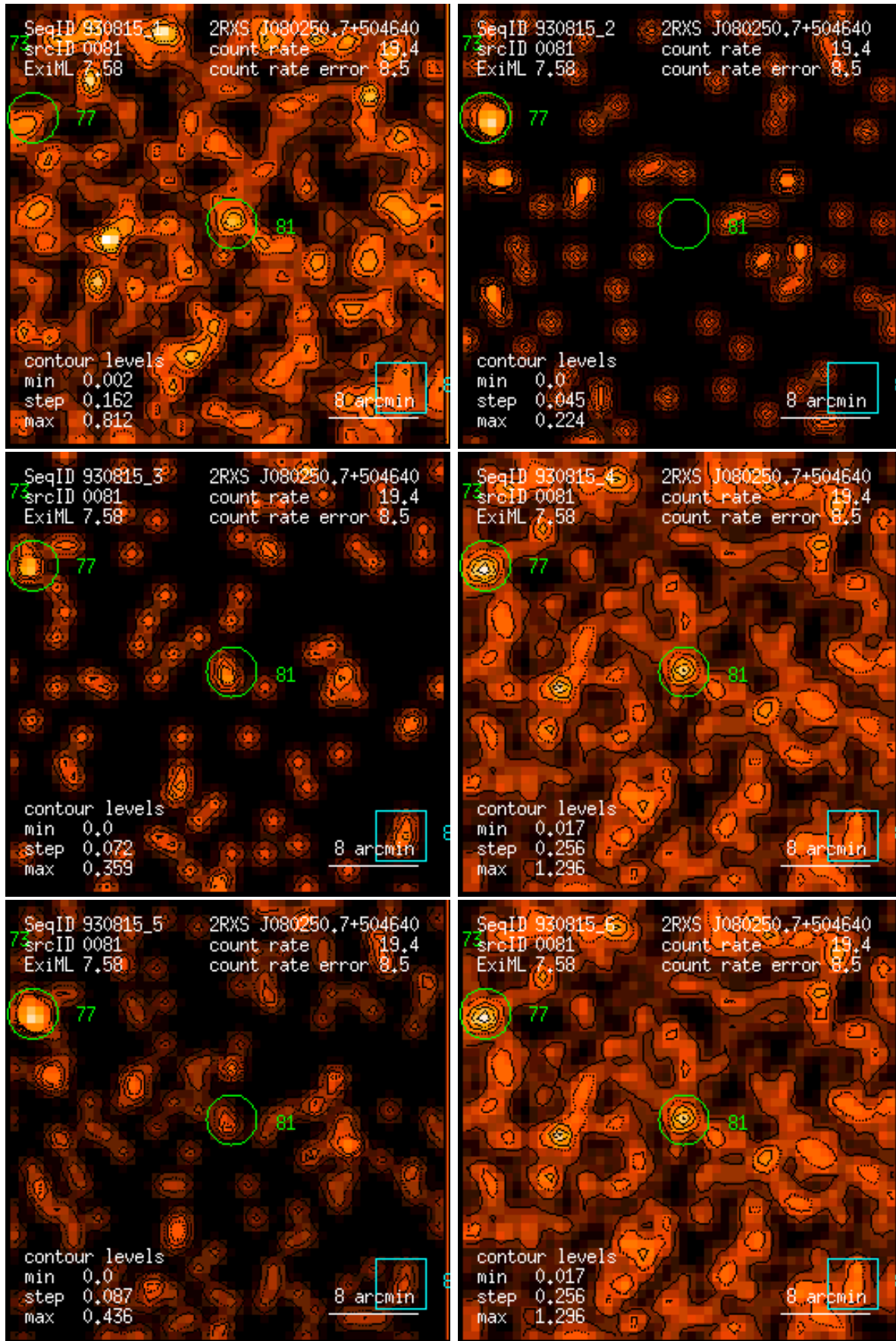
Figure 81: RASS 930815: detection 0081: band rate images, Gaussian filter: (1) PSPC channels 11 – 41, (2) 52 – 90, (3) 91 – 201, (4) 11 – 235, (5) 52 – 201, (6) 11 – 201. Broad band rates in counts/ks. Band rate contour levels in counts/ks/arcmin 2 .
