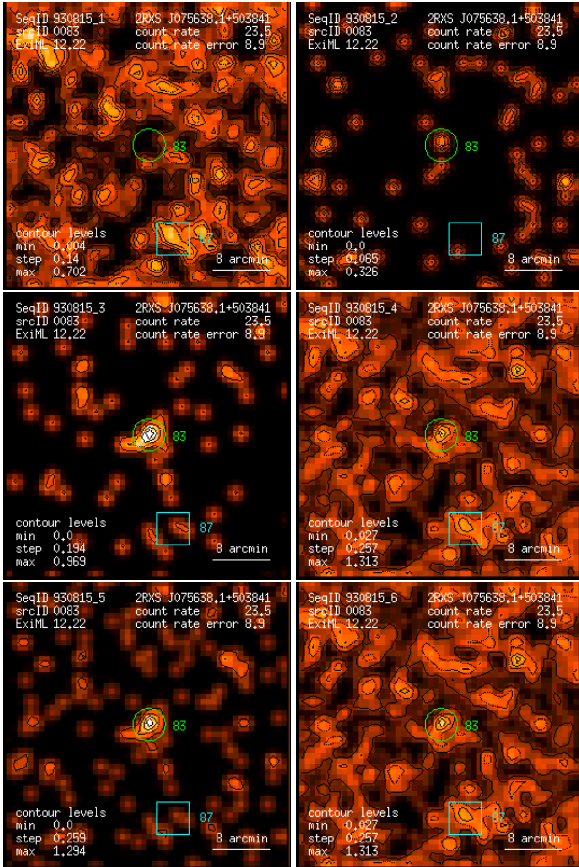
Figure 83: RASS 930815: detection 0083: band rate images, Gaussian filter: (1) PSPC channels 11 – 41, (2) 52 – 90, (3) 91 – 201, (4) 11 – 235, (5) 52 – 201, (6) 11 – 201. Broad band rates in counts/ks. Band rate contour levels in counts/ks/arcmin 2 .
