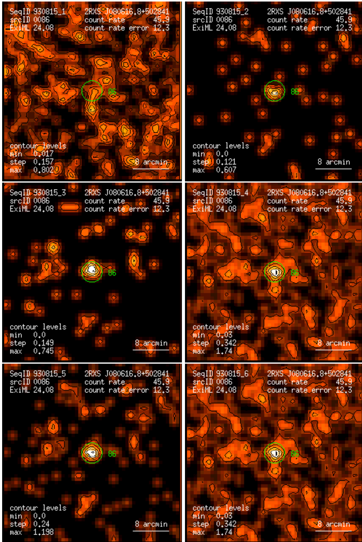
Figure 86: RASS 930815: detection 0086: band rate images, Gaussian filter: (1) PSPC channels 11 – 41, (2) 52 – 90, (3) 91 – 201, (4) 11 – 235, (5) 52 – 201, (6) 11 – 201. Broad band rates in counts/ks. Band rate contour levels in counts/ks/arcmin 2 .
