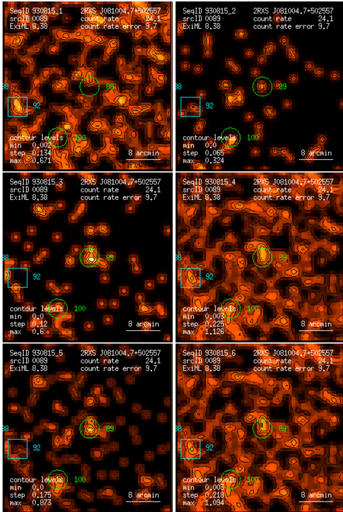
Figure 89: RASS 930815: detection 0089: band rate images, Gaussian filter: (1) PSPC channels 11 – 41, (2) 52 – 90, (3) 91 – 201, (4) 11 – 235, (5) 52 – 201, (6) 11 – 201. Broad band rates in counts/ks. Band rate contour levels in counts/ks/arcmin 2 .
