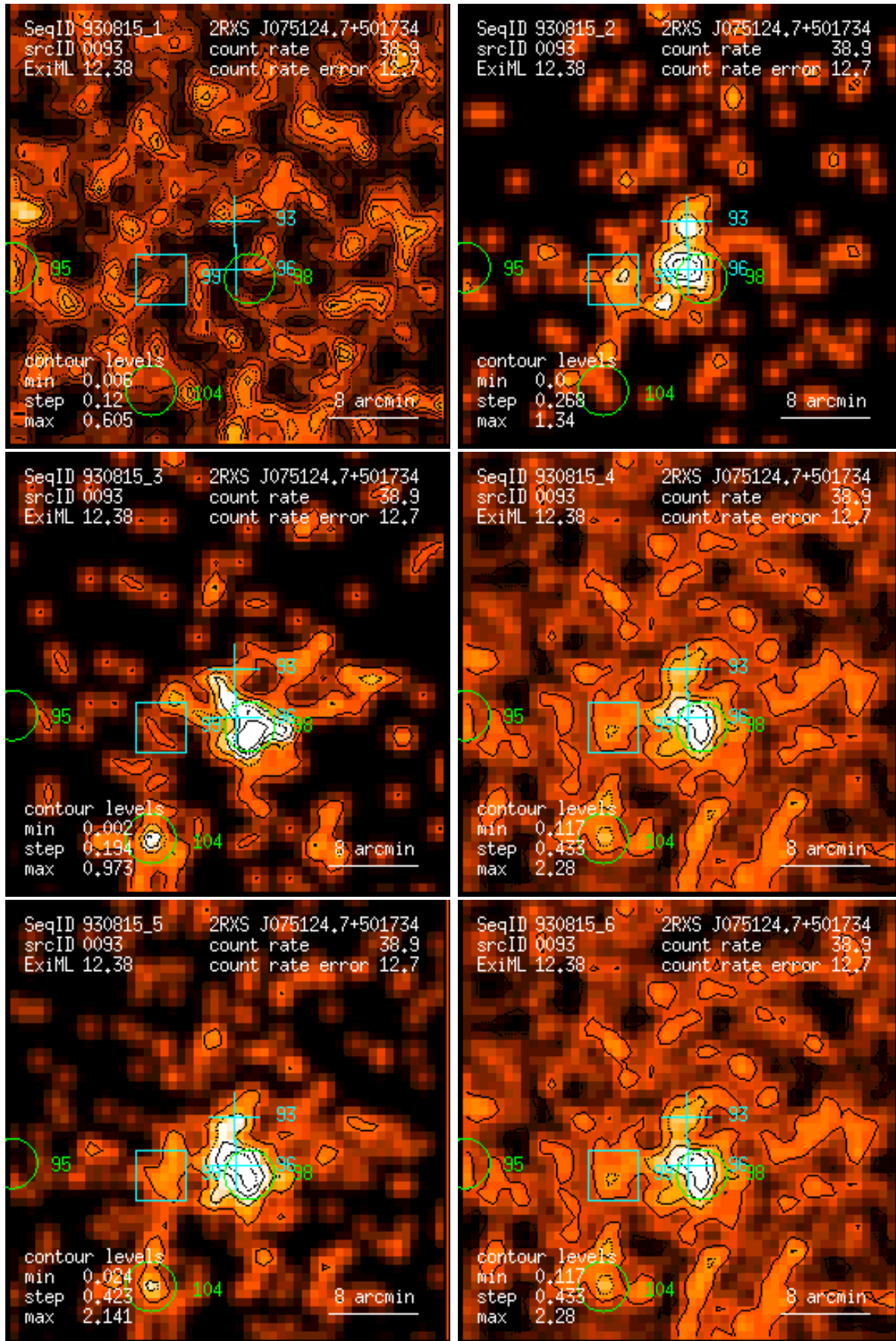
Figure 93: RASS 930815: detection 0093: band rate images, Gaussian filter: (1) PSPC channels 11 – 41, (2) 52 – 90, (3) 91 – 201, (4) 11 – 235, (5) 52 – 201, (6) 11 – 201. Broad band rates in counts/ks. Band rate contour levels in counts/ks/arcmin 2 .
