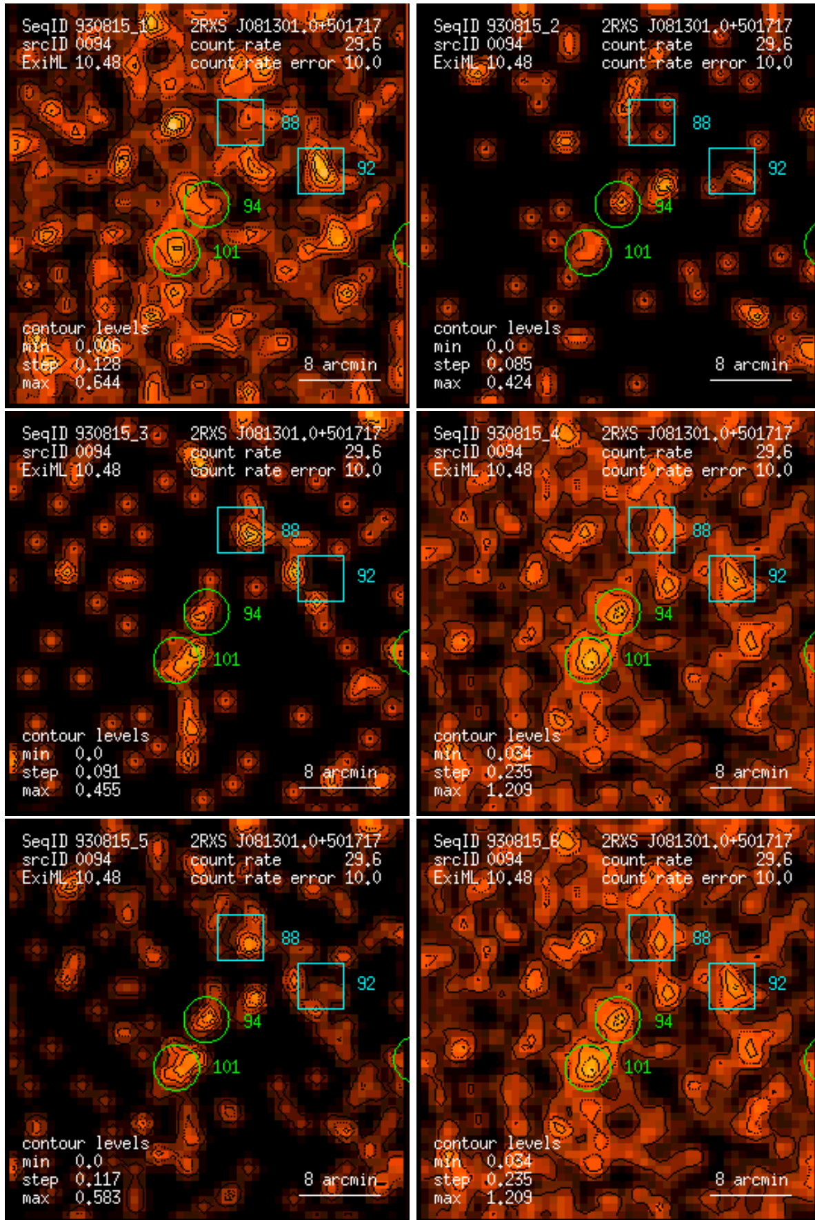
Figure 94: RASS 930815: detection 0094: band rate images, Gaussian filter: (1) PSPC channels 11 – 41, (2) 52 – 90, (3) 91 – 201, (4) 11 – 235, (5) 52 – 201, (6) 11 – 201. Broad band rates in counts/ks. Band rate contour levels in counts/ks/arcmin 2 .
