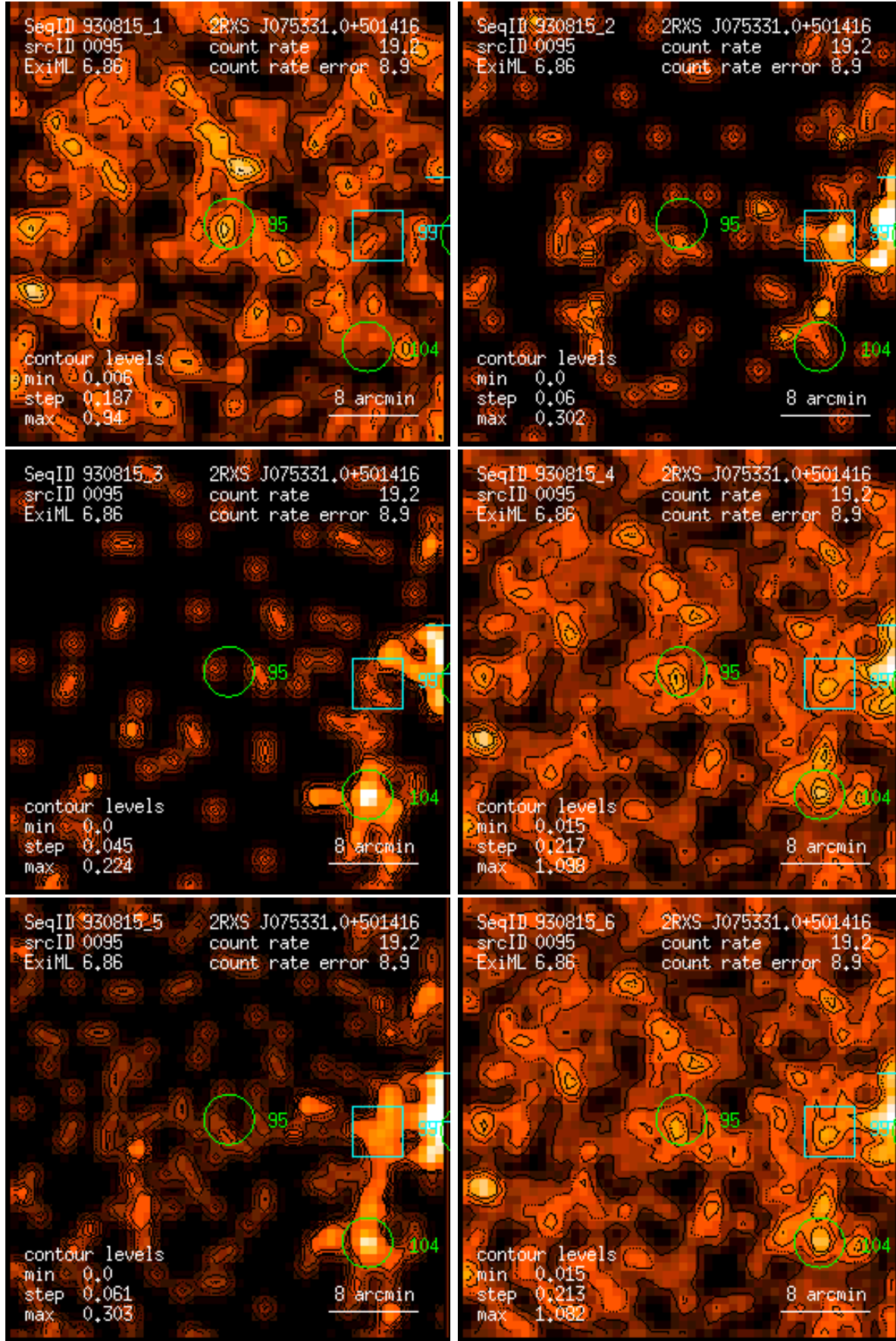
Figure 95: RASS 930815: detection 0095: band rate images, Gaussian filter: (1) PSPC channels 11 – 41, (2) 52 – 90, (3) 91 – 201, (4) 11 – 235, (5) 52 – 201, (6) 11 – 201. Broad band rates in counts/ks. Band rate contour levels in counts/ks/arcmin 2 .
