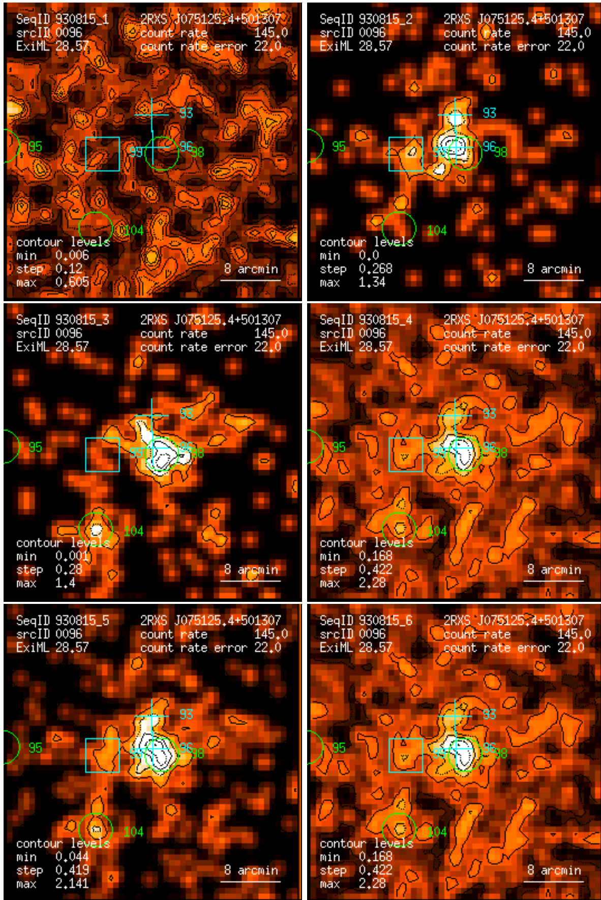
Figure 96: RASS 930815: detection 0096: band rate images, Gaussian filter: (1) PSPC channels 11 – 41, (2) 52 – 90, (3) 91 – 201, (4) 11 – 235, (5) 52 – 201, (6) 11 – 201. Broad band rates in counts/ks. Band rate contour levels in counts/ks/arcmin 2 .
