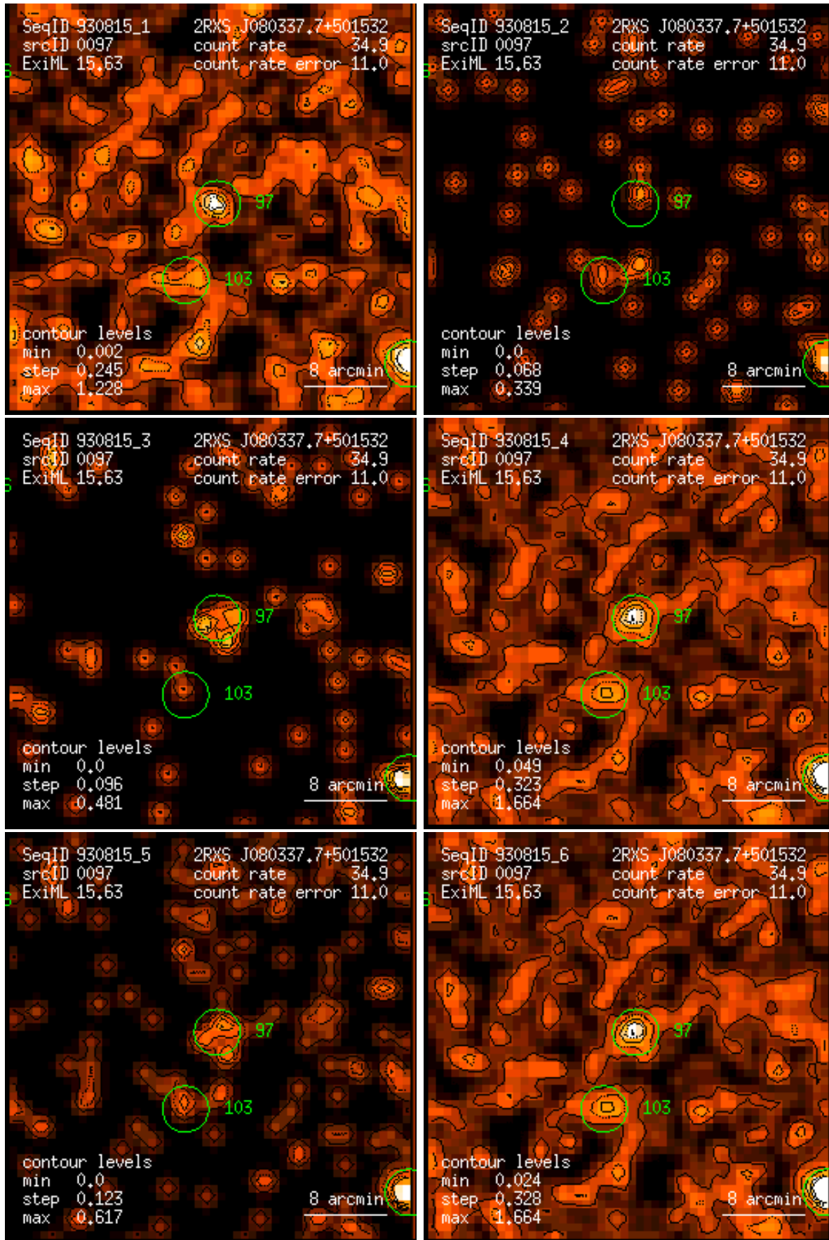
Figure 97: RASS 930815: detection 0097: band rate images, Gaussian filter: (1) PSPC channels 11 – 41, (2) 52 – 90, (3) 91 – 201, (4) 11 – 235, (5) 52 – 201, (6) 11 – 201. Broad band rates in counts/ks. Band rate contour levels in counts/ks/arcmin 2 .
