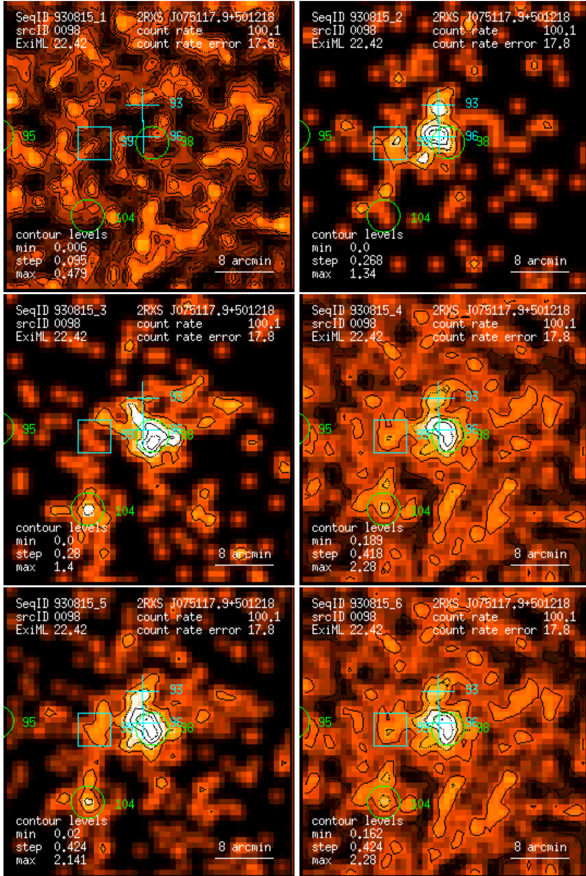
Figure 98: RASS 930815: detection 0098: band rate images, Gaussian filter: (1) PSPC channels 11 – 41, (2) 52 – 90, (3) 91 – 201, (4) 11 – 235, (5) 52 – 201, (6) 11 – 201. Broad band rates in counts/ks. Band rate contour levels in counts/ks/arcmin 2 .
