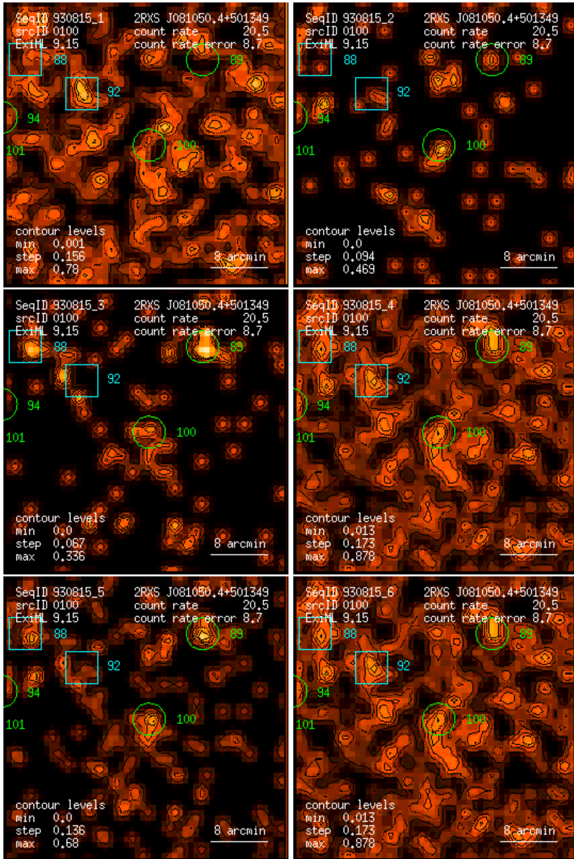
Figure 100: RASS 930815: detection 0100: band rate images, Gaussian filter: (1) PSPC channels 11 – 41, (2) 52 – 90, (3) 91 – 201, (4) 11 – 235, (5) 52 – 201, (6) 11 – 201. Broad band rates in counts/ks. Band rate contour levels in counts/ks/arcmin 2 .
