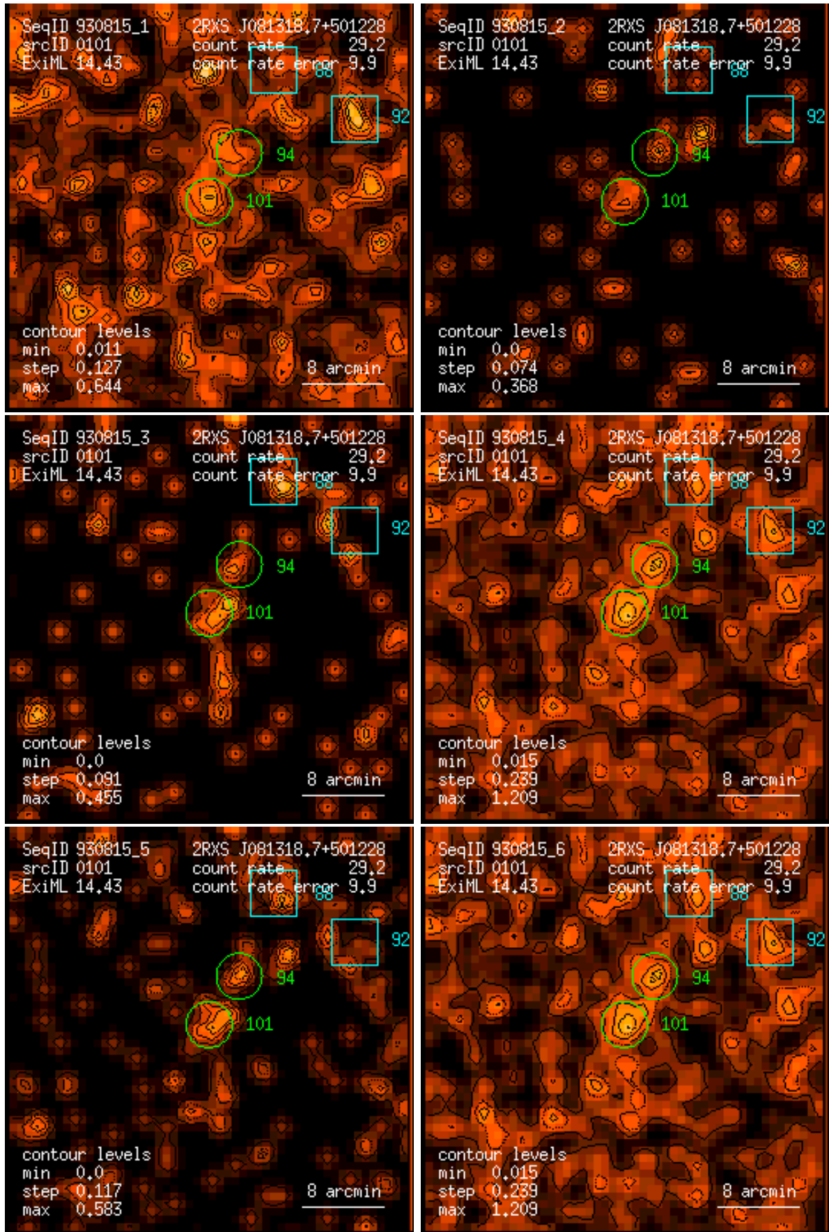
Figure 101: RASS 930815: detection 0101: band rate images, Gaussian filter: (1) PSPC channels 11 – 41, (2) 52 – 90, (3) 91 – 201, (4) 11 – 235, (5) 52 – 201, (6) 11 – 201. Broad band rates in counts/ks. Band rate contour levels in counts/ks/arcmin 2 .
