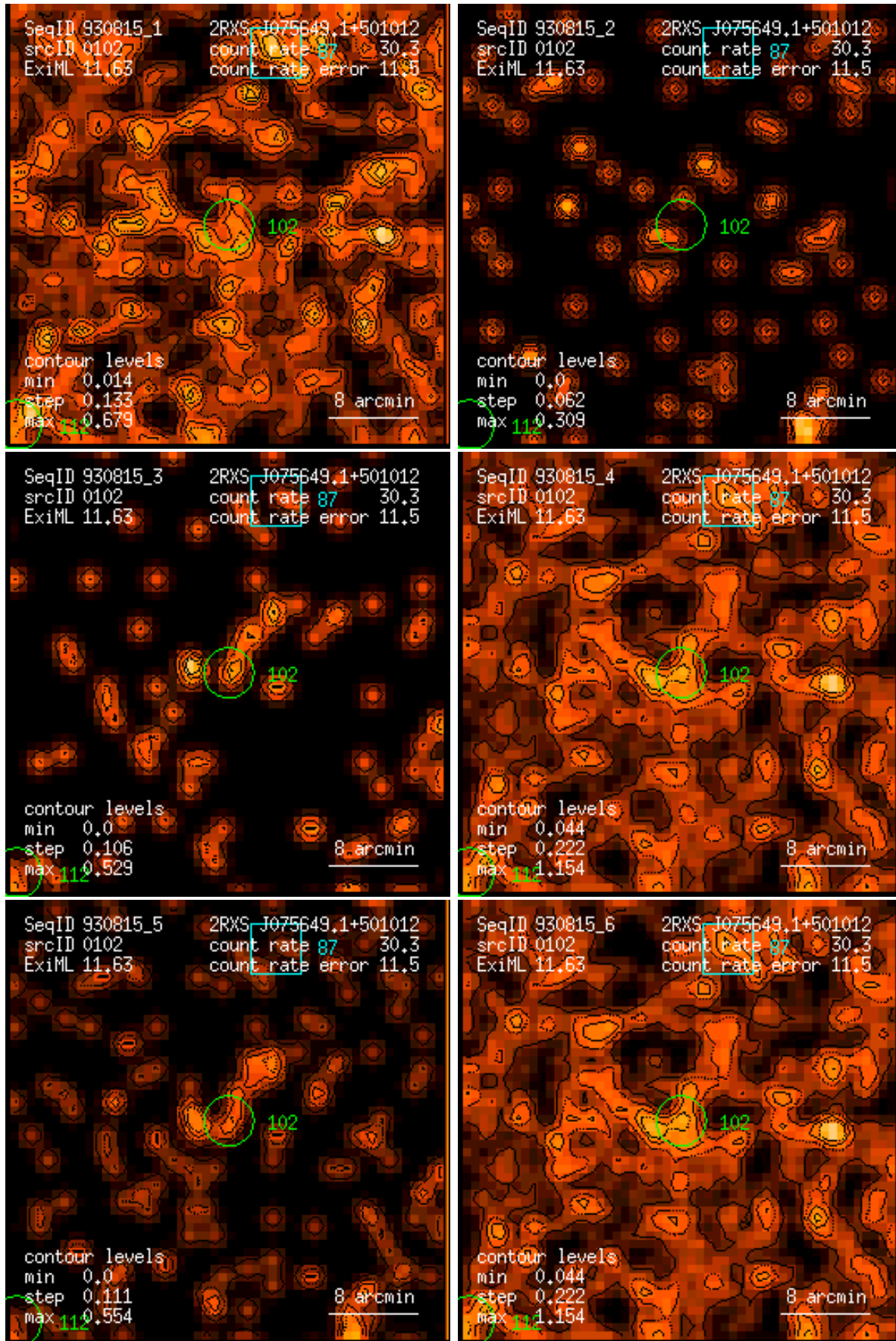
Figure 102: RASS 930815: detection 0102: band rate images, Gaussian filter: (1) PSPC channels 11 – 41, (2) 52 – 90, (3) 91 – 201, (4) 11 – 235, (5) 52 – 201, (6) 11 – 201. Broad band rates in counts/ks. Band rate contour levels in counts/ks/arcmin 2 .
