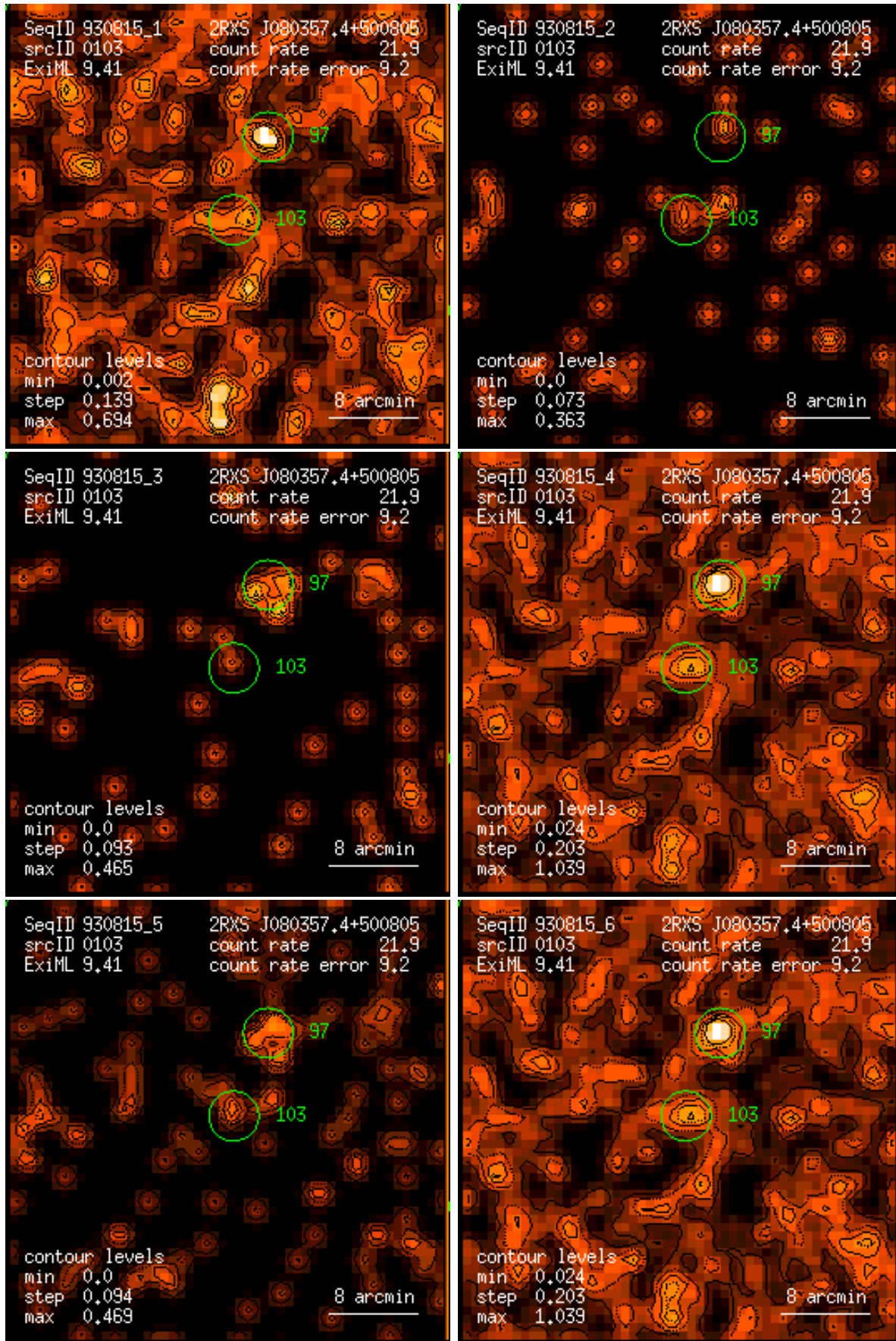
Figure 103: RASS 930815: detection 0103: band rate images, Gaussian filter: (1) PSPC channels 11 – 41, (2) 52 – 90, (3) 91 – 201, (4) 11 – 235, (5) 52 – 201, (6) 11 – 201. Broad band rates in counts/ks. Band rate contour levels in counts/ks/arcmin 2 .
