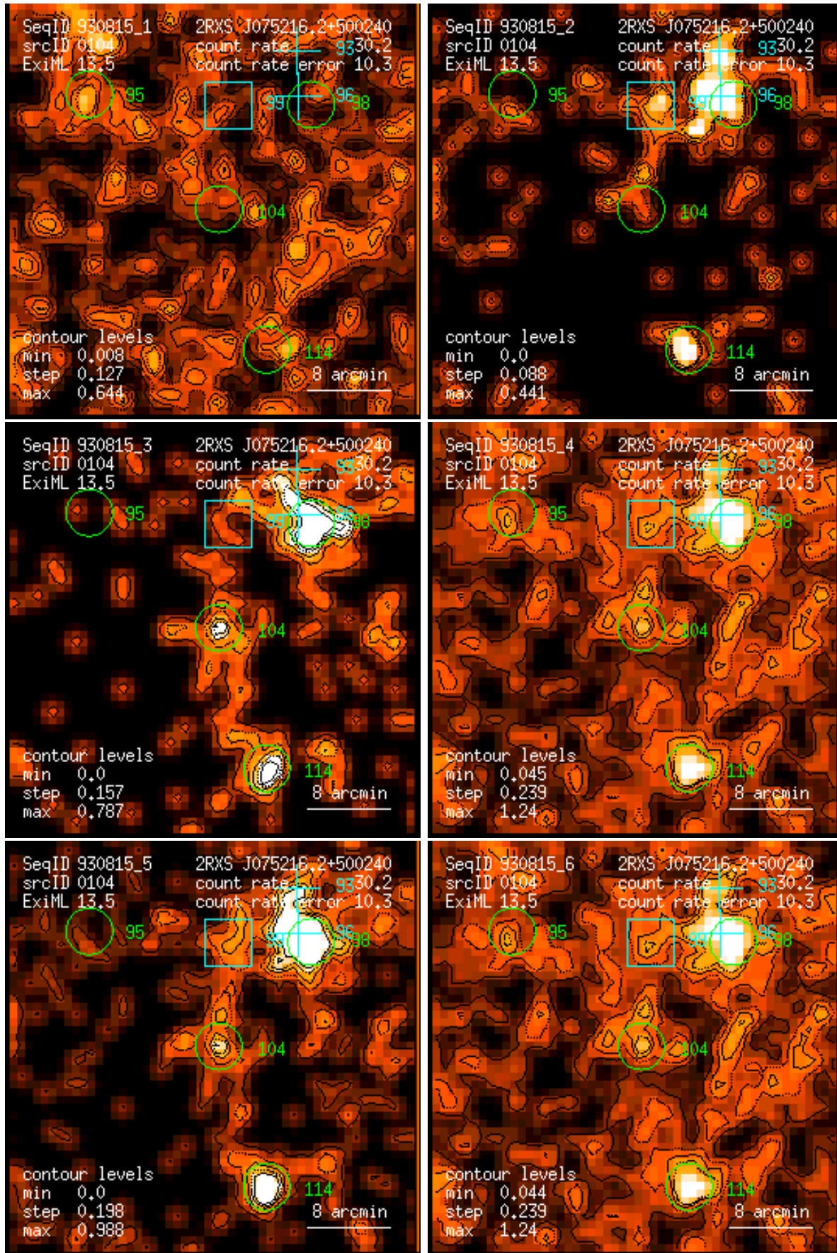
Figure 104: RASS 930815: detection 0104: band rate images, Gaussian filter: (1) PSPC channels 11 – 41, (2) 52 – 90, (3) 91 – 201, (4) 11 – 235, (5) 52 – 201, (6) 11 – 201. Broad band rates in counts/ks. Band rate contour levels in counts/ks/arcmin 2 .
