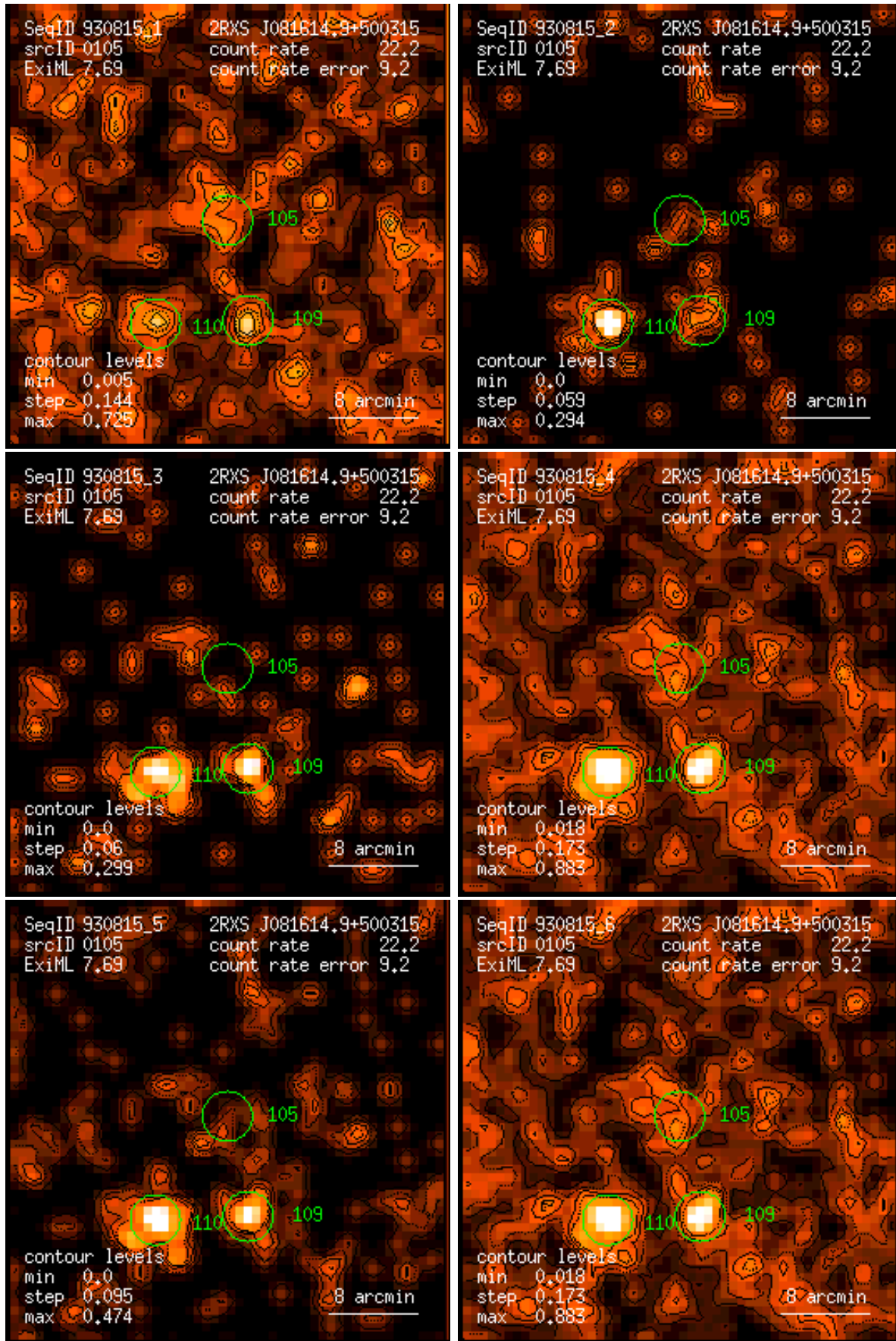
Figure 105: RASS 930815: detection 0105: band rate images, Gaussian filter: (1) PSPC channels 11 – 41, (2) 52 – 90, (3) 91 – 201, (4) 11 – 235, (5) 52 – 201, (6) 11 – 201. Broad band rates in counts/ks. Band rate contour levels in counts/ks/arcmin 2 .
