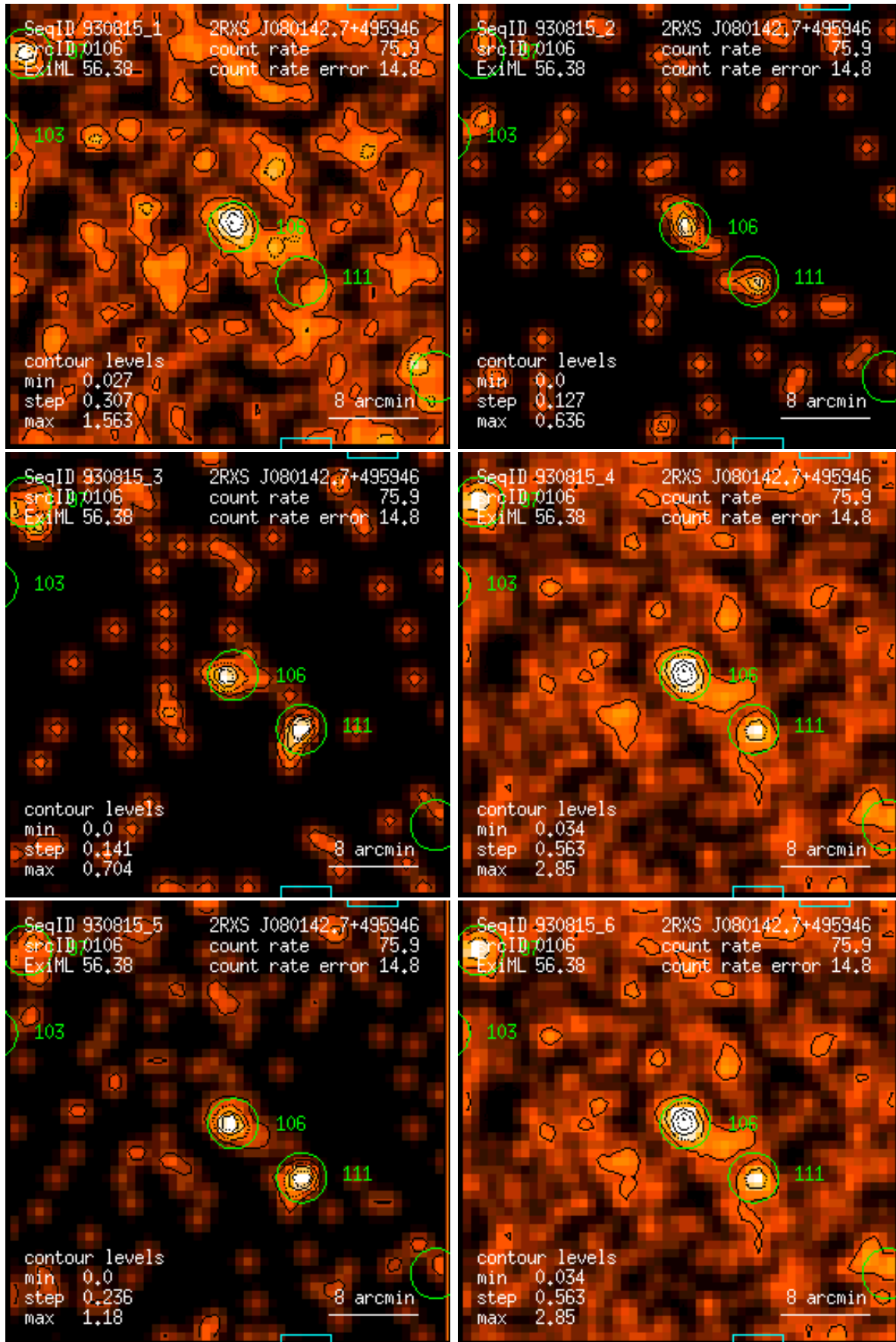
Figure 106: RASS 930815: detection 0106: band rate images, Gaussian filter: (1) PSPC channels 11 – 41, (2) 52 – 90, (3) 91 – 201, (4) 11 – 235, (5) 52 – 201, (6) 11 – 201. Broad band rates in counts/ks. Band rate contour levels in counts/ks/arcmin 2 .
