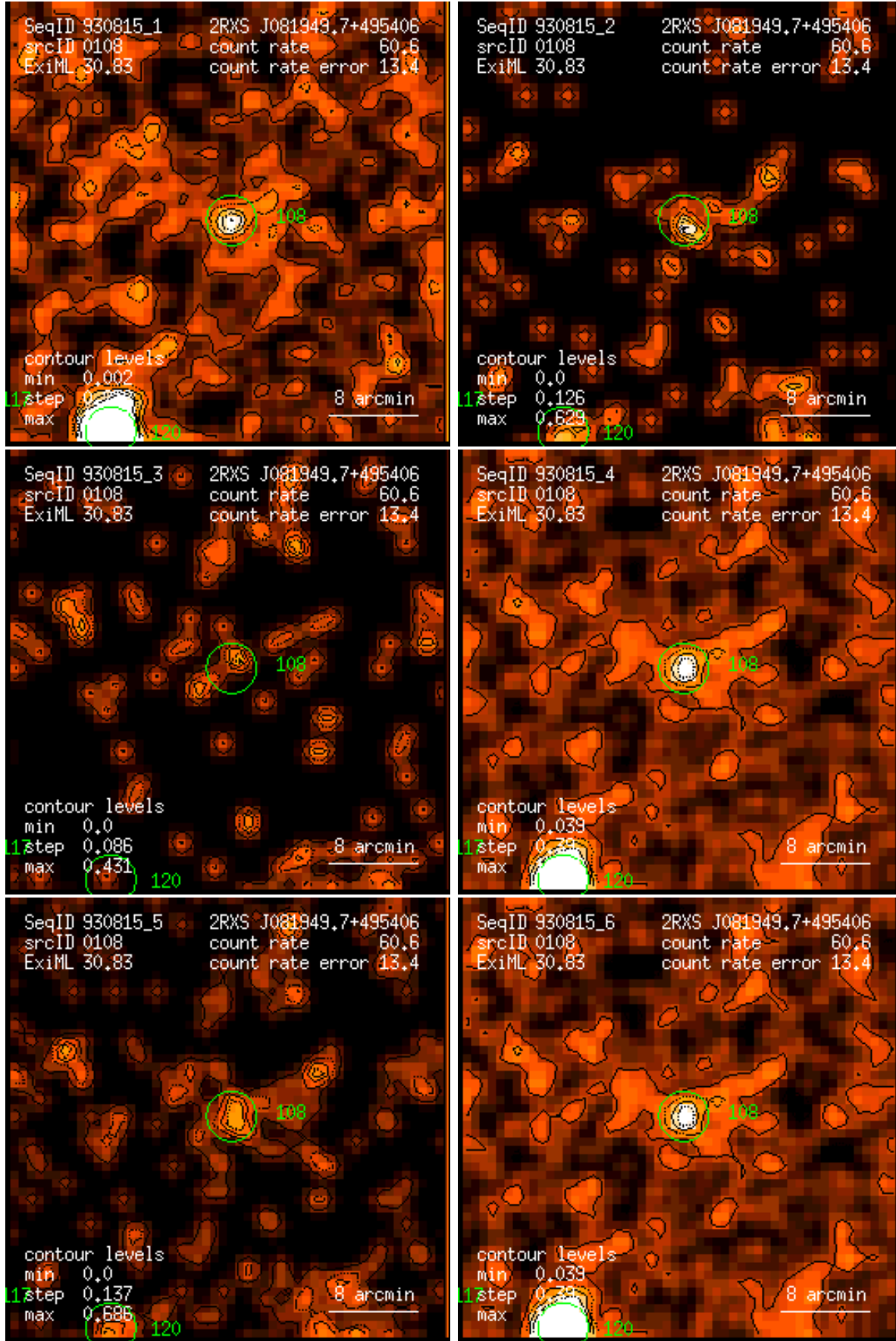
Figure 108: RASS 930815: detection 0108: band rate images, Gaussian filter: (1) PSPC channels 11 – 41, (2) 52 – 90, (3) 91 – 201, (4) 11 – 235, (5) 52 – 201, (6) 11 – 201. Broad band rates in counts/ks. Band rate contour levels in counts/ks/arcmin 2 .
