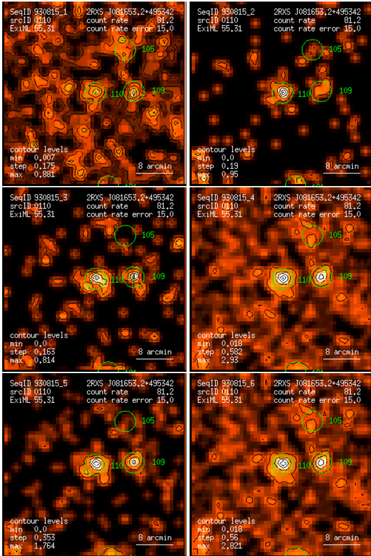
Figure 110: RASS 930815: detection 0110: band rate images, Gaussian filter: (1) PSPC channels 11 – 41, (2) 52 – 90, (3) 91 – 201, (4) 11 – 235, (5) 52 – 201, (6) 11 – 201. Broad band rates in counts/ks. Band rate contour levels in counts/ks/arcmin 2 .
