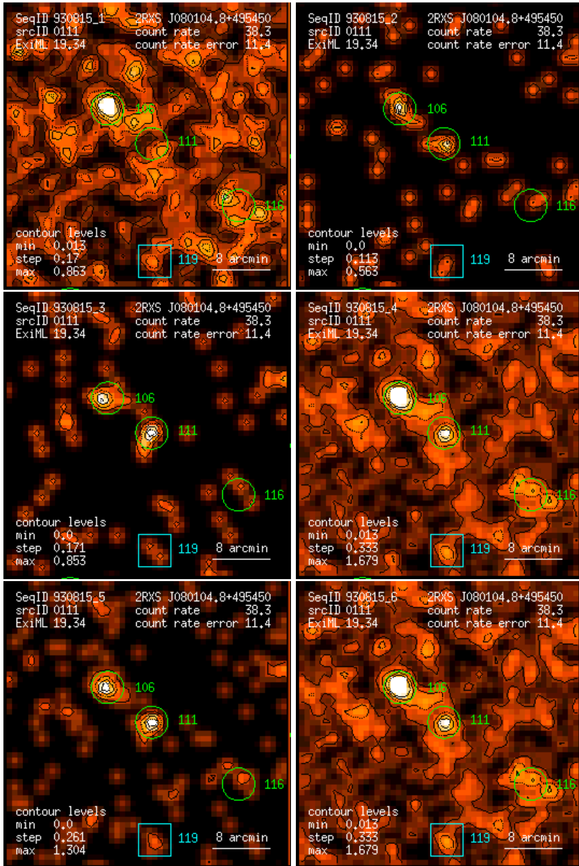
Figure 111: RASS 930815: detection 0111: band rate images, Gaussian filter: (1) PSPC channels 11 – 41, (2) 52 – 90, (3) 91 – 201, (4) 11 – 235, (5) 52 – 201, (6) 11 – 201. Broad band rates in counts/ks. Band rate contour levels in counts/ks/arcmin 2 .
