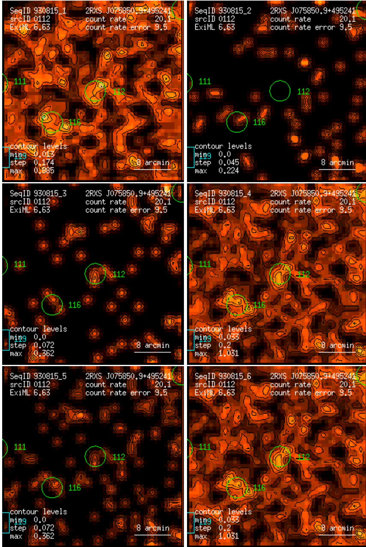
Figure 112: RASS 930815: detection 0112: band rate images, Gaussian filter: (1) PSPC channels 11 – 41, (2) 52 – 90, (3) 91 – 201, (4) 11 – 235, (5) 52 – 201, (6) 11 – 201. Broad band rates in counts/ks. Band rate contour levels in counts/ks/arcmin 2 .
