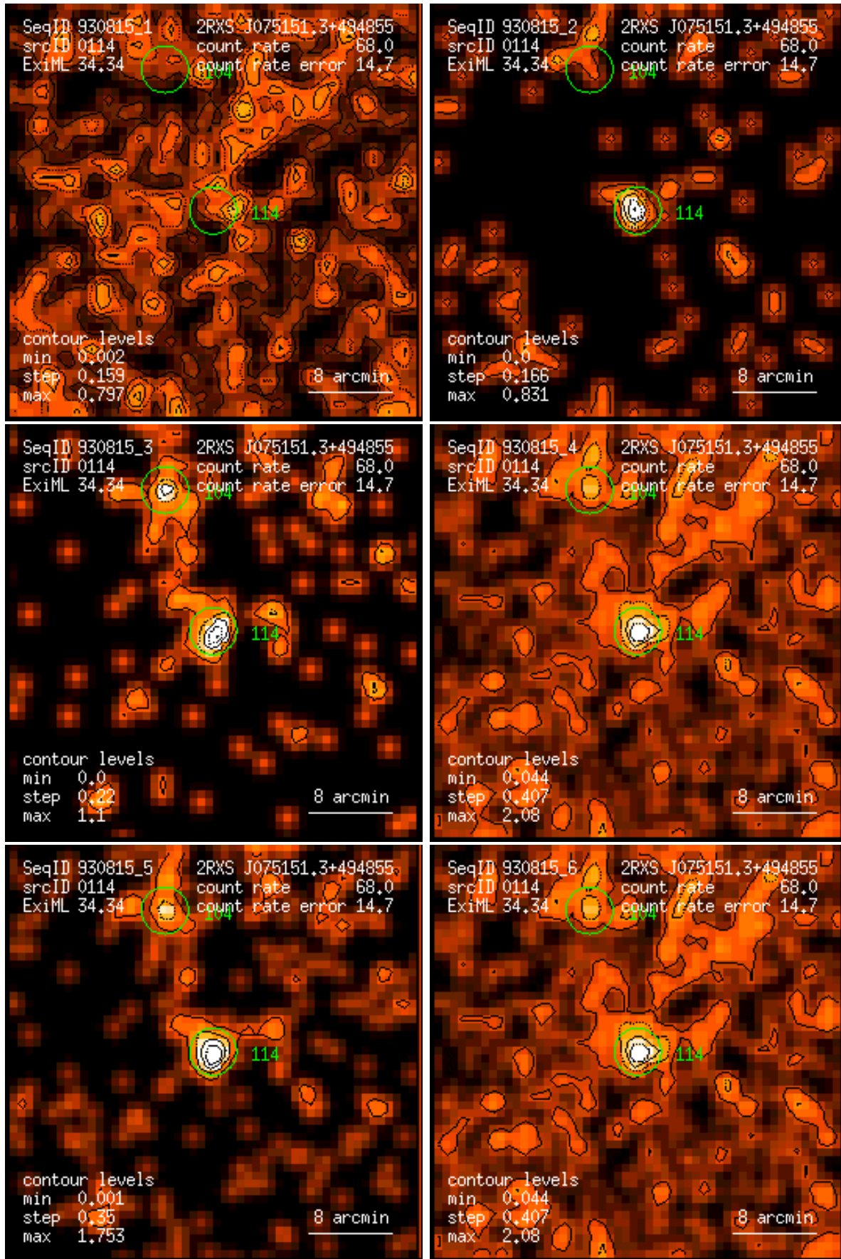
Figure 114: RASS 930815: detection 0114: band rate images, Gaussian filter: (1) PSPC channels 11 – 41, (2) 52 – 90, (3) 91 – 201, (4) 11 – 235, (5) 52 – 201, (6) 11 – 201. Broad band rates in counts/ks. Band rate contour levels in counts/ks/arcmin 2 .
