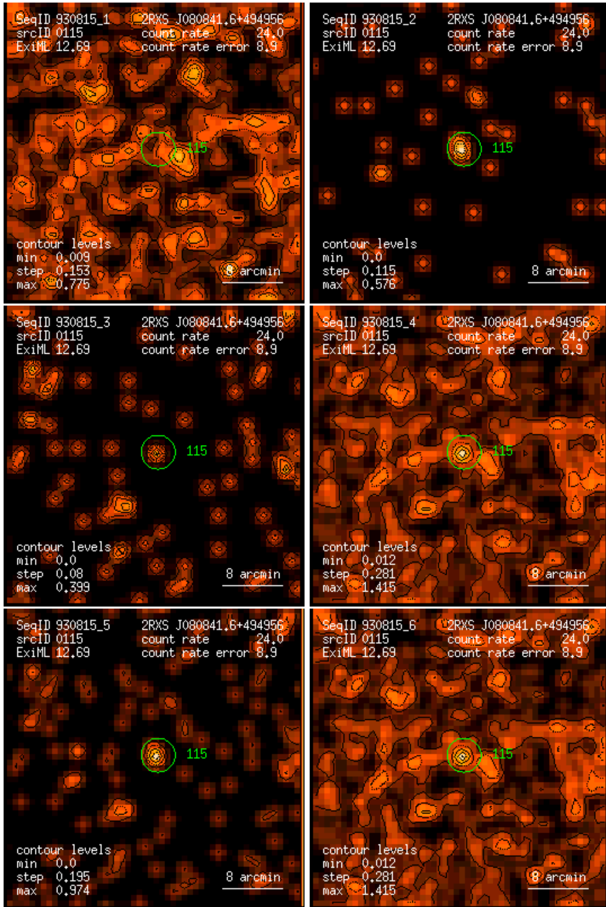
Figure 115: RASS 930815: detection 0115: band rate images, Gaussian filter: (1) PSPC channels 11 – 41, (2) 52 – 90, (3) 91 – 201, (4) 11 – 235, (5) 52 – 201, (6) 11 – 201. Broad band rates in counts/ks. Band rate contour levels in counts/ks/arcmin 2 .
