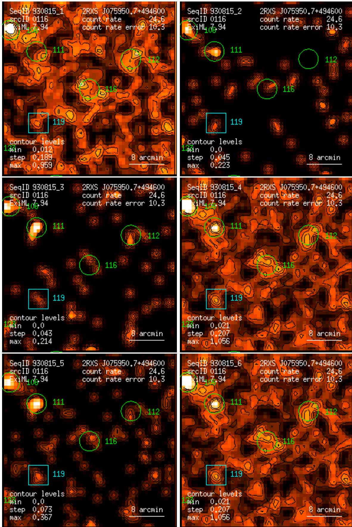
Figure 116: RASS 930815: detection 0116: band rate images, Gaussian filter: (1) PSPC channels 11 – 41, (2) 52 – 90, (3) 91 – 201, (4) 11 – 235, (5) 52 – 201, (6) 11 – 201. Broad band rates in counts/ks. Band rate contour levels in counts/ks/arcmin 2 .
