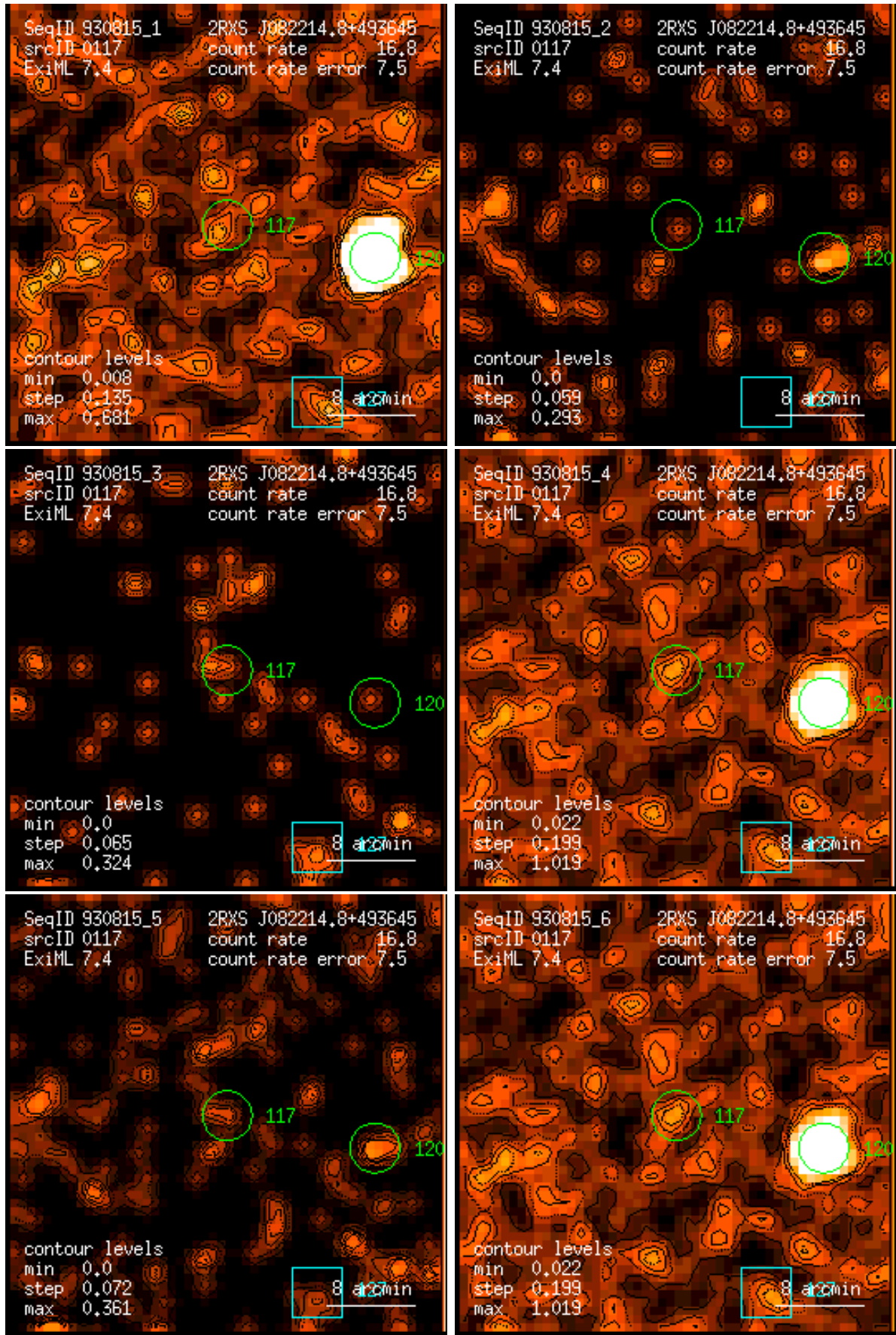
Figure 117: RASS 930815: detection 0117: band rate images, Gaussian filter: (1) PSPC channels 11 – 41, (2) 52 – 90, (3) 91 – 201, (4) 11 – 235, (5) 52 – 201, (6) 11 – 201. Broad band rates in counts/ks. Band rate contour levels in counts/ks/arcmin 2 .
