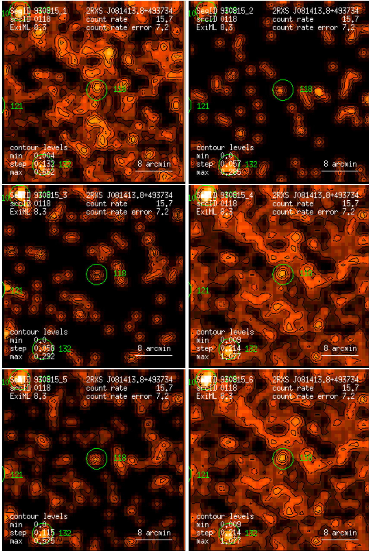
Figure 118: RASS 930815: detection 0118: band rate images, Gaussian filter: (1) PSPC channels 11 – 41, (2) 52 – 90, (3) 91 – 201, (4) 11 – 235, (5) 52 – 201, (6) 11 – 201. Broad band rates in counts/ks. Band rate contour levels in counts/ks/arcmin 2 .
