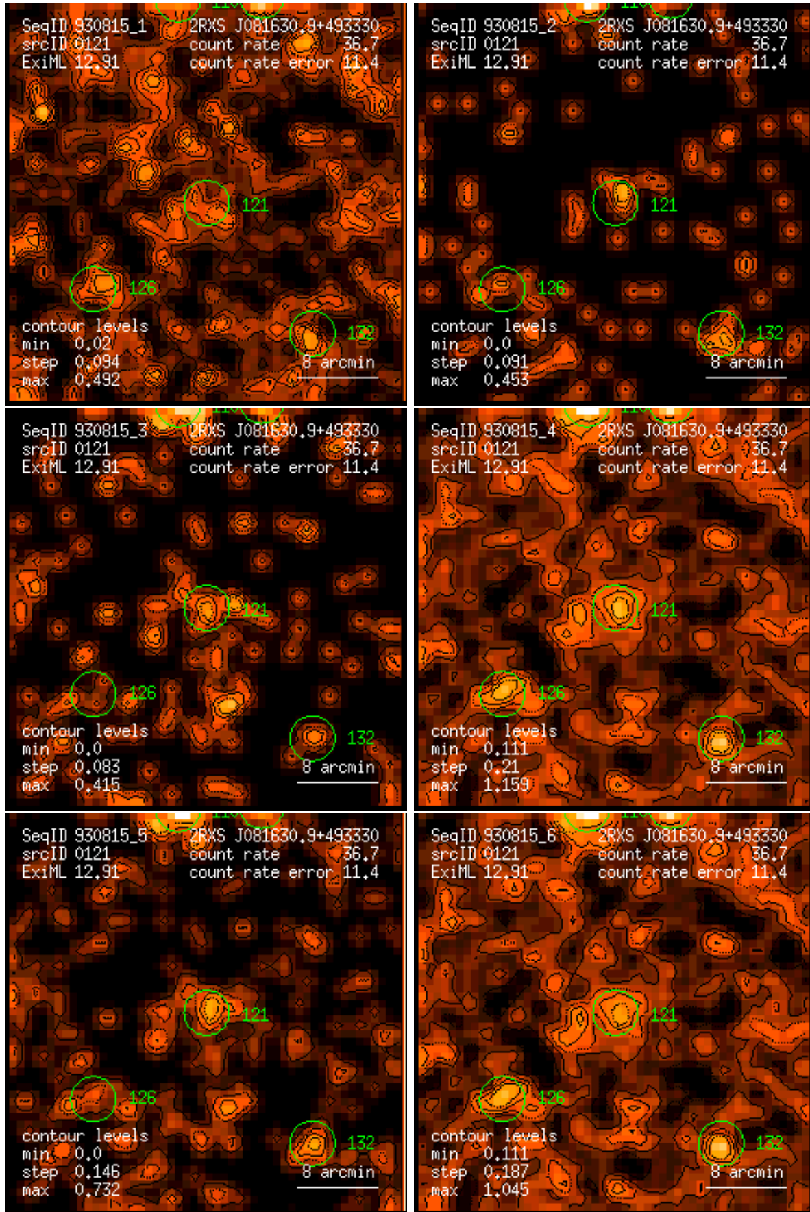
Figure 121: RASS 930815: detection 0121: band rate images, Gaussian filter: (1) PSPC channels 11 – 41, (2) 52 – 90, (3) 91 – 201, (4) 11 – 235, (5) 52 – 201, (6) 11 – 201. Broad band rates in counts/ks. Band rate contour levels in counts/ks/arcmin 2 .
