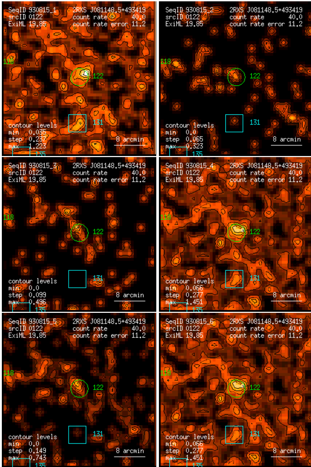
Figure 122: RASS 930815: detection 0122: band rate images, Gaussian filter: (1) PSPC channels 11 – 41, (2) 52 – 90, (3) 91 – 201, (4) 11 – 235, (5) 52 – 201, (6) 11 – 201. Broad band rates in counts/ks. Band rate contour levels in counts/ks/arcmin 2 .
