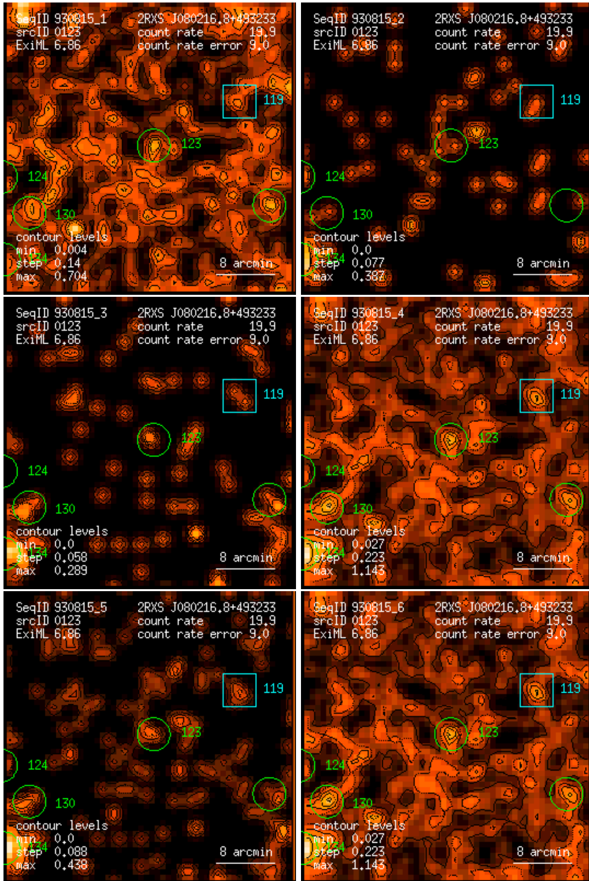
Figure 123: RASS 930815: detection 0123: band rate images, Gaussian filter: (1) PSPC channels 11 – 41, (2) 52 – 90, (3) 91 – 201, (4) 11 – 235, (5) 52 – 201, (6) 11 – 201. Broad band rates in counts/ks. Band rate contour levels in counts/ks/arcmin 2 .
