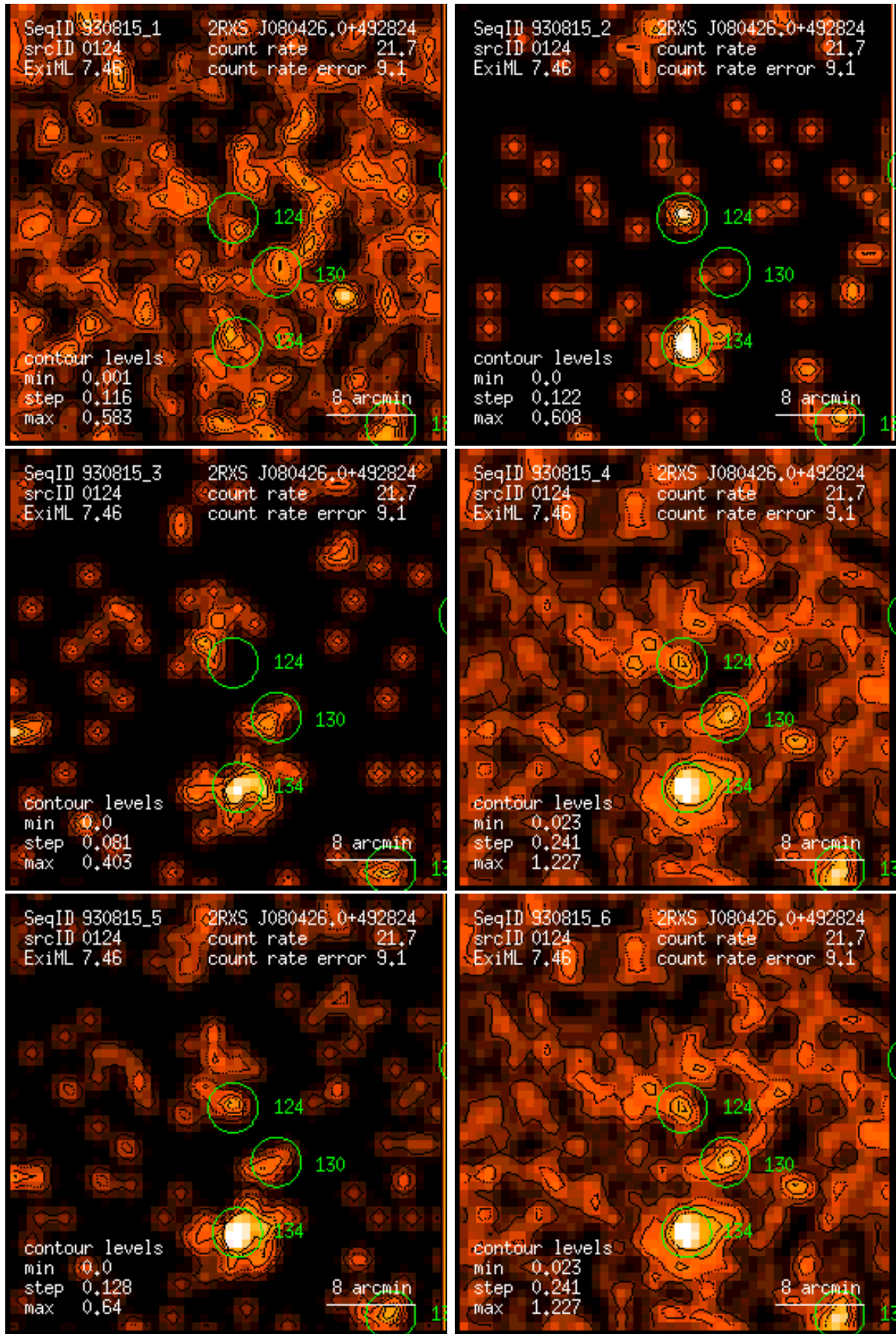
Figure 124: RASS 930815: detection 0124: band rate images, Gaussian filter: (1) PSPC channels 11 – 41, (2) 52 – 90, (3) 91 – 201, (4) 11 – 235, (5) 52 – 201, (6) 11 – 201. Broad band rates in counts/ks. Band rate contour levels in counts/ks/arcmin 2 .
