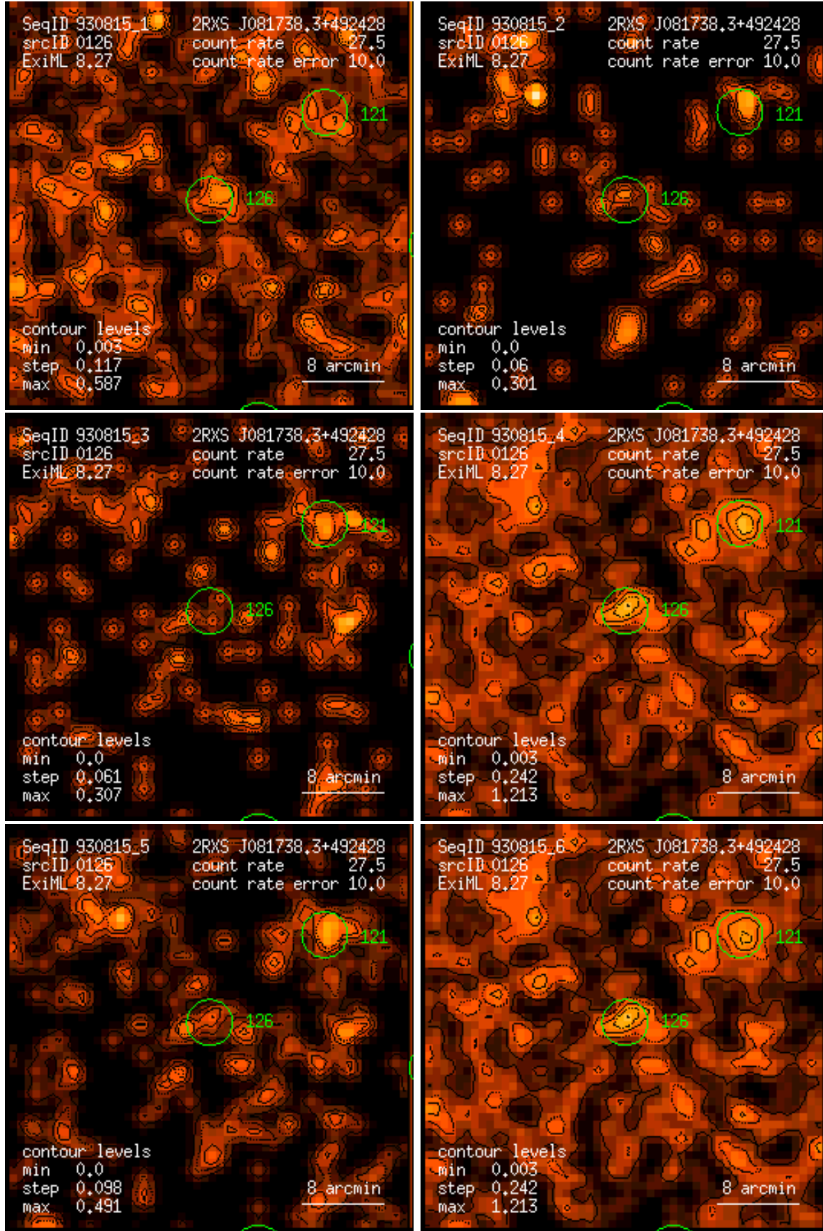
Figure 126: RASS 930815: detection 0126: band rate images, Gaussian filter: (1) PSPC channels 11 – 41, (2) 52 – 90, (3) 91 – 201, (4) 11 – 235, (5) 52 – 201, (6) 11 – 201. Broad band rates in counts/ks. Band rate contour levels in counts/ks/arcmin 2 .
