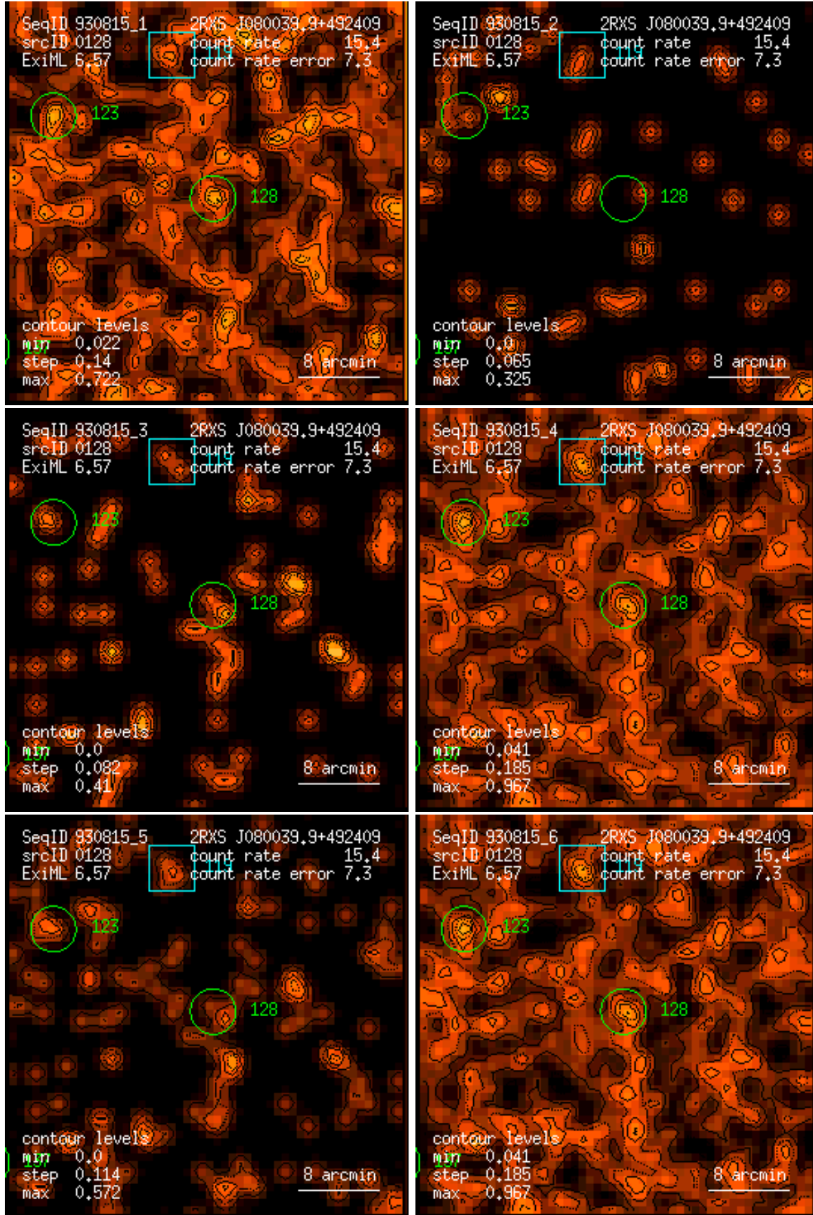
Figure 128: RASS 930815: detection 0128: band rate images, Gaussian filter: (1) PSPC channels 11 – 41, (2) 52 – 90, (3) 91 – 201, (4) 11 – 235, (5) 52 – 201, (6) 11 – 201. Broad band rates in counts/ks. Band rate contour levels in counts/ks/arcmin 2 .
