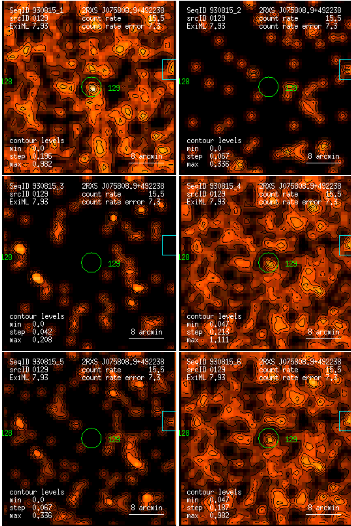
Figure 129: RASS 930815: detection 0129: band rate images, Gaussian filter: (1) PSPC channels 11 – 41, (2) 52 – 90, (3) 91 – 201, (4) 11 – 235, (5) 52 – 201, (6) 11 – 201. Broad band rates in counts/ks. Band rate contour levels in counts/ks/arcmin 2 .
