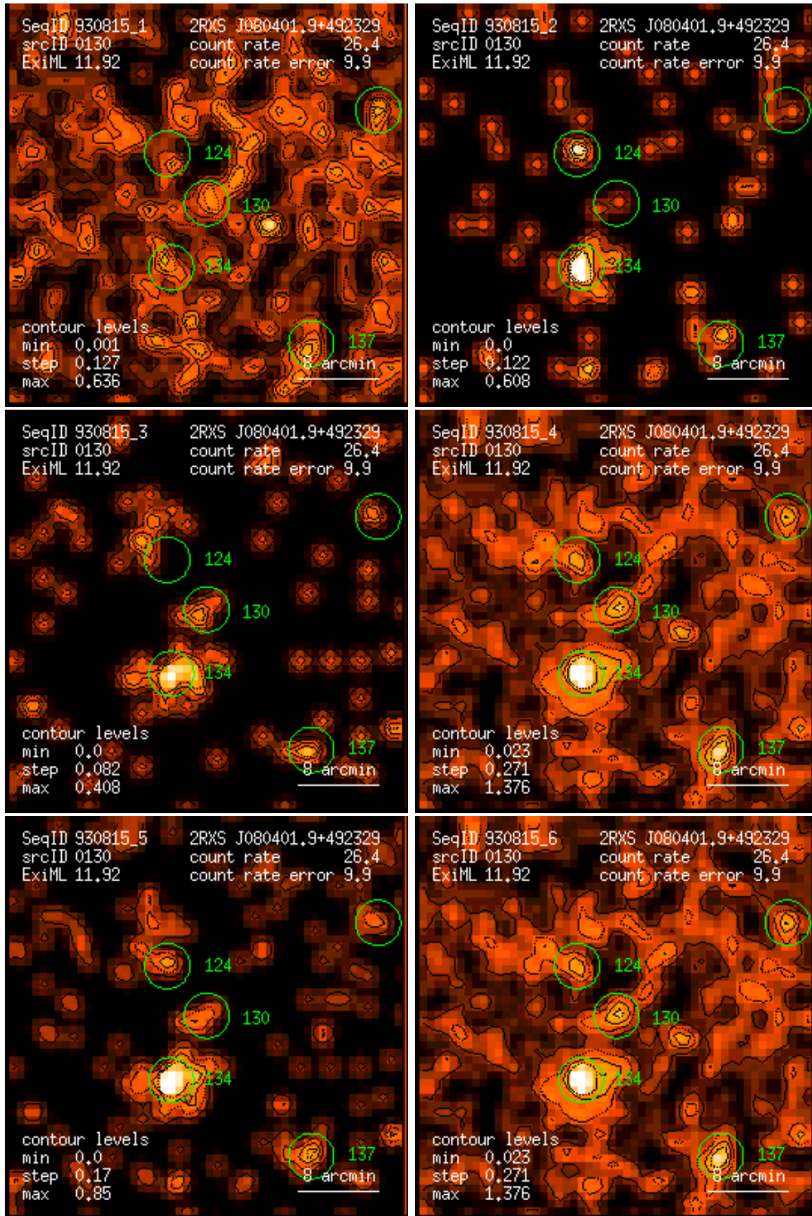
Figure 130: RASS 930815: detection 0130: band rate images, Gaussian filter: (1) PSPC channels 11 – 41, (2) 52 – 90, (3) 91 – 201, (4) 11 – 235, (5) 52 – 201, (6) 11 – 201. Broad band rates in counts/ks. Band rate contour levels in counts/ks/arcmin 2 .
