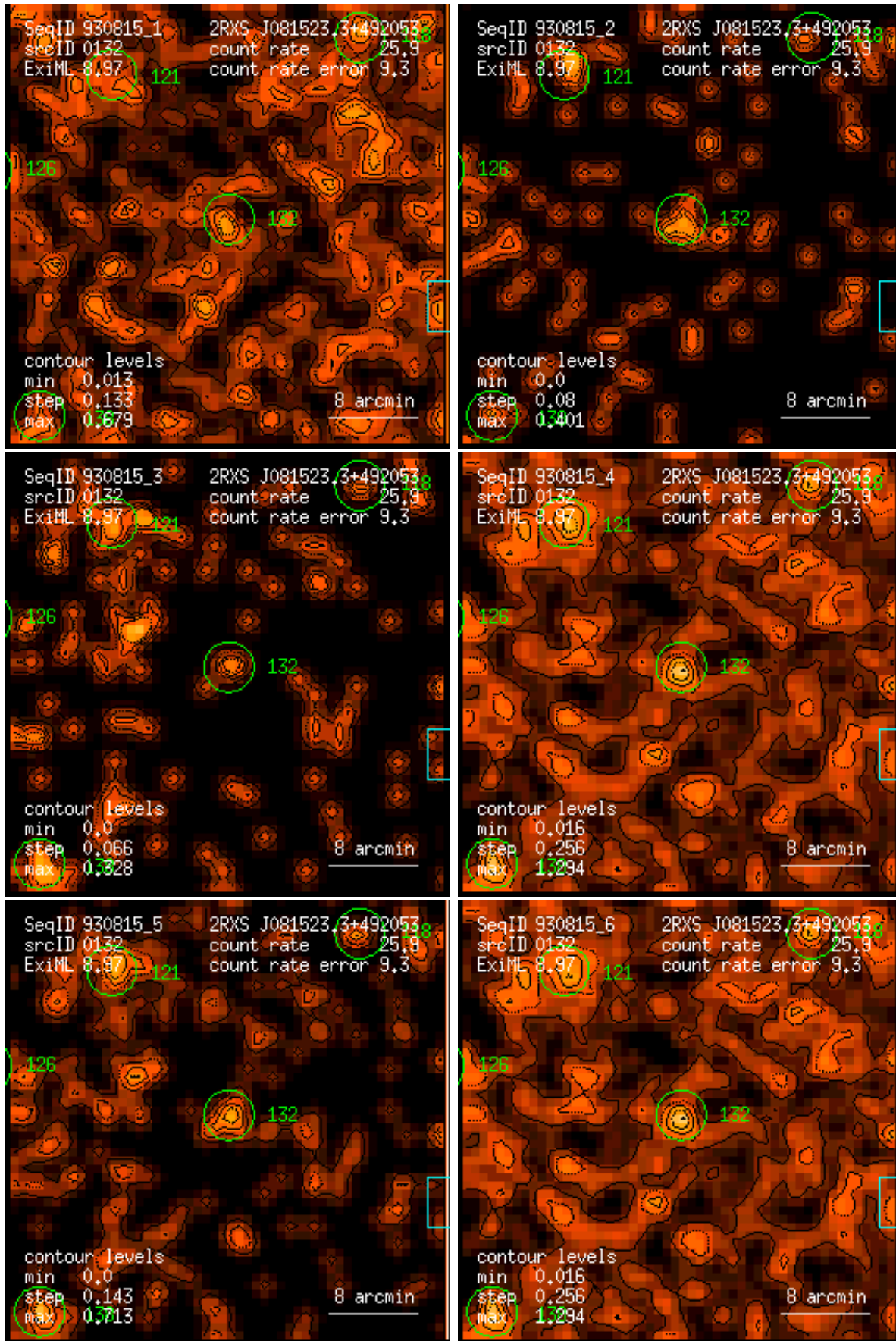
Figure 132: RASS 930815: detection 0132: band rate images, Gaussian filter: (1) PSPC channels 11 – 41, (2) 52 – 90, (3) 91 – 201, (4) 11 – 235, (5) 52 – 201, (6) 11 – 201. Broad band rates in counts/ks. Band rate contour levels in counts/ks/arcmin 2 .
