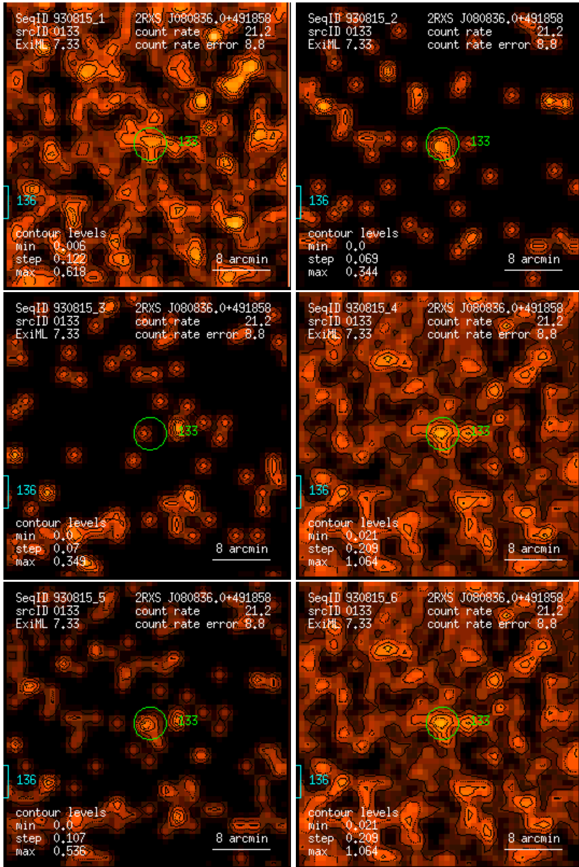
Figure 133: RASS 930815: detection 0133: band rate images, Gaussian filter: (1) PSPC channels 11 – 41, (2) 52 – 90, (3) 91 – 201, (4) 11 – 235, (5) 52 – 201, (6) 11 – 201. Broad band rates in counts/ks. Band rate contour levels in counts/ks/arcmin 2 .
