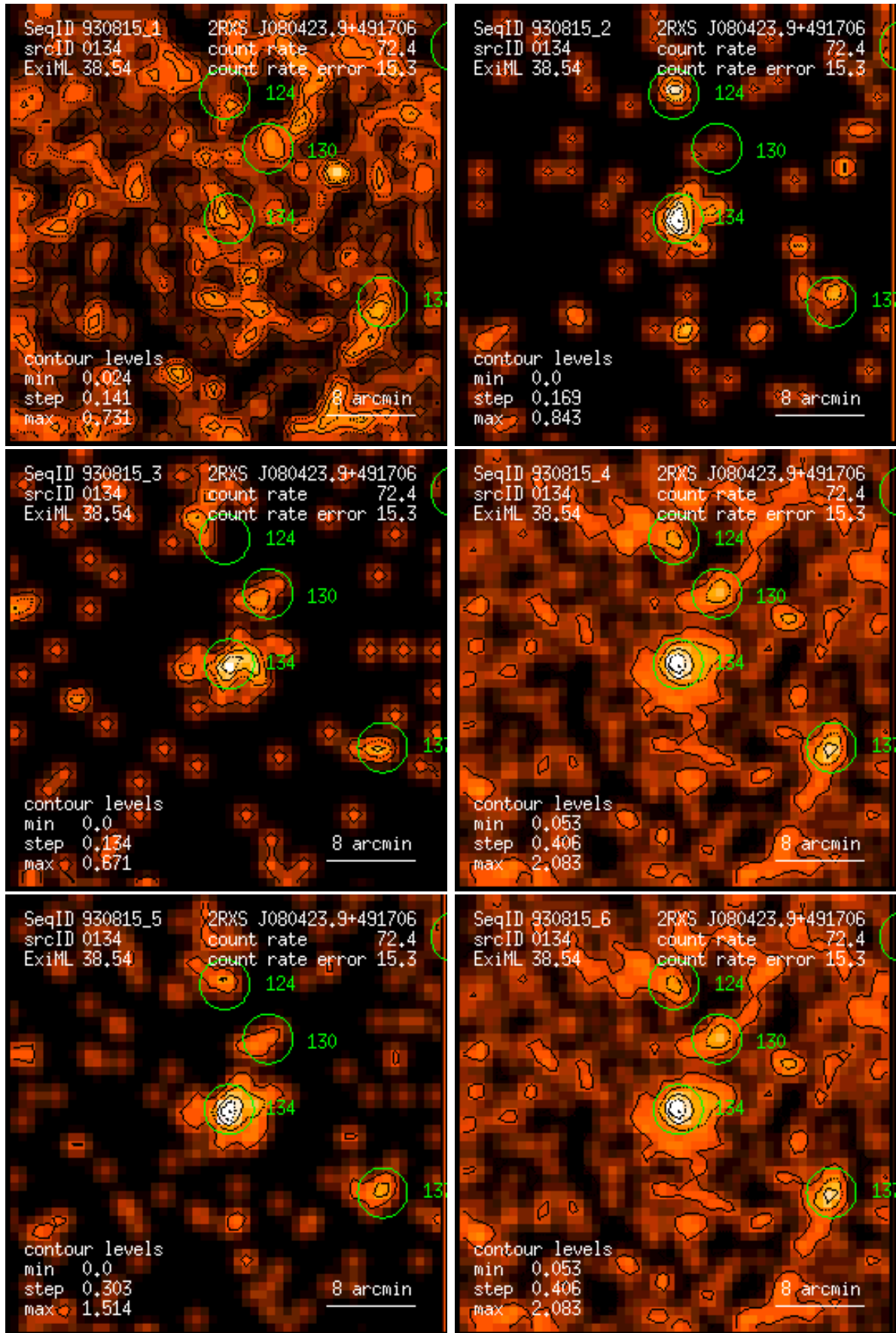
Figure 134: RASS 930815: detection 0134: band rate images, Gaussian filter: (1) PSPC channels 11 – 41, (2) 52 – 90, (3) 91 – 201, (4) 11 – 235, (5) 52 – 201, (6) 11 – 201. Broad band rates in counts/ks. Band rate contour levels in counts/ks/arcmin 2 .
