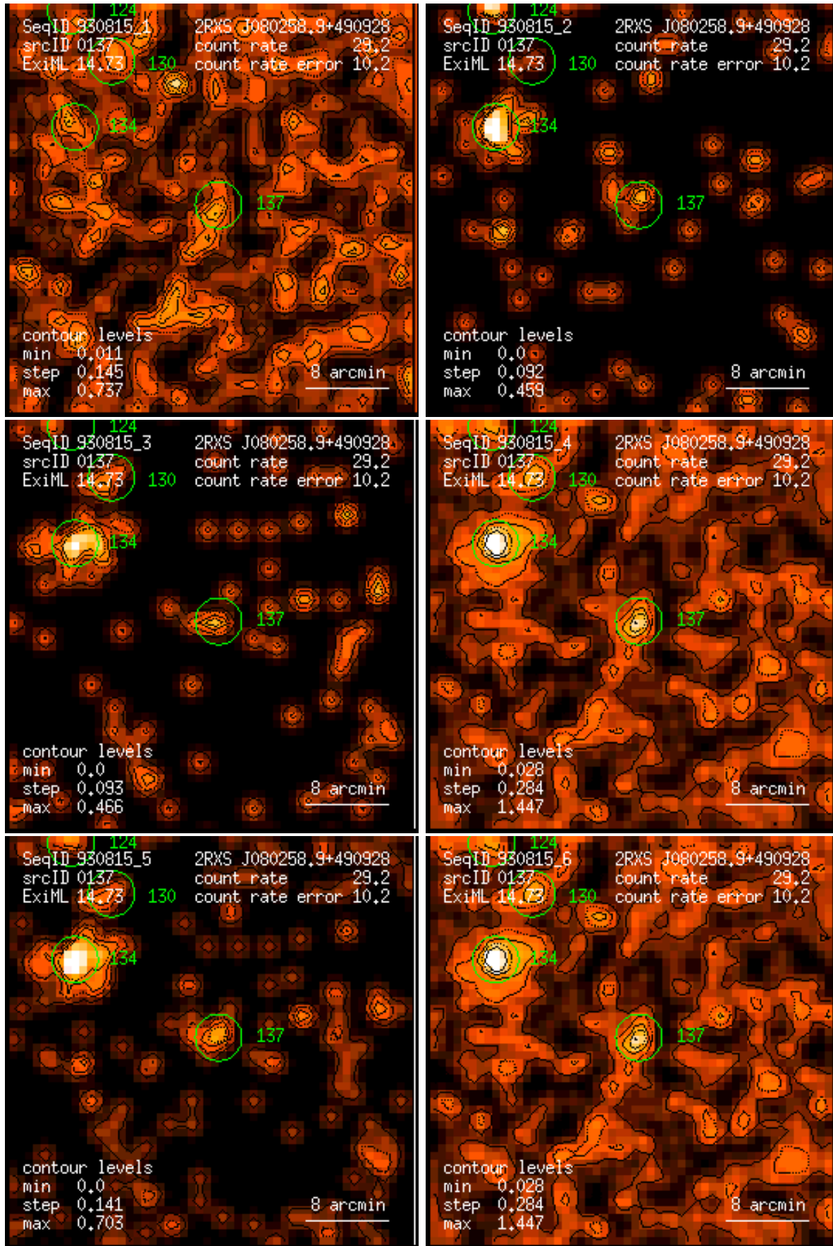
Figure 137: RASS 930815: detection 0137: band rate images, Gaussian filter: (1) PSPC channels 11 – 41, (2) 52 – 90, (3) 91 – 201, (4) 11 – 235, (5) 52 – 201, (6) 11 – 201. Broad band rates in counts/ks. Band rate contour levels in counts/ks/arcmin 2 .
