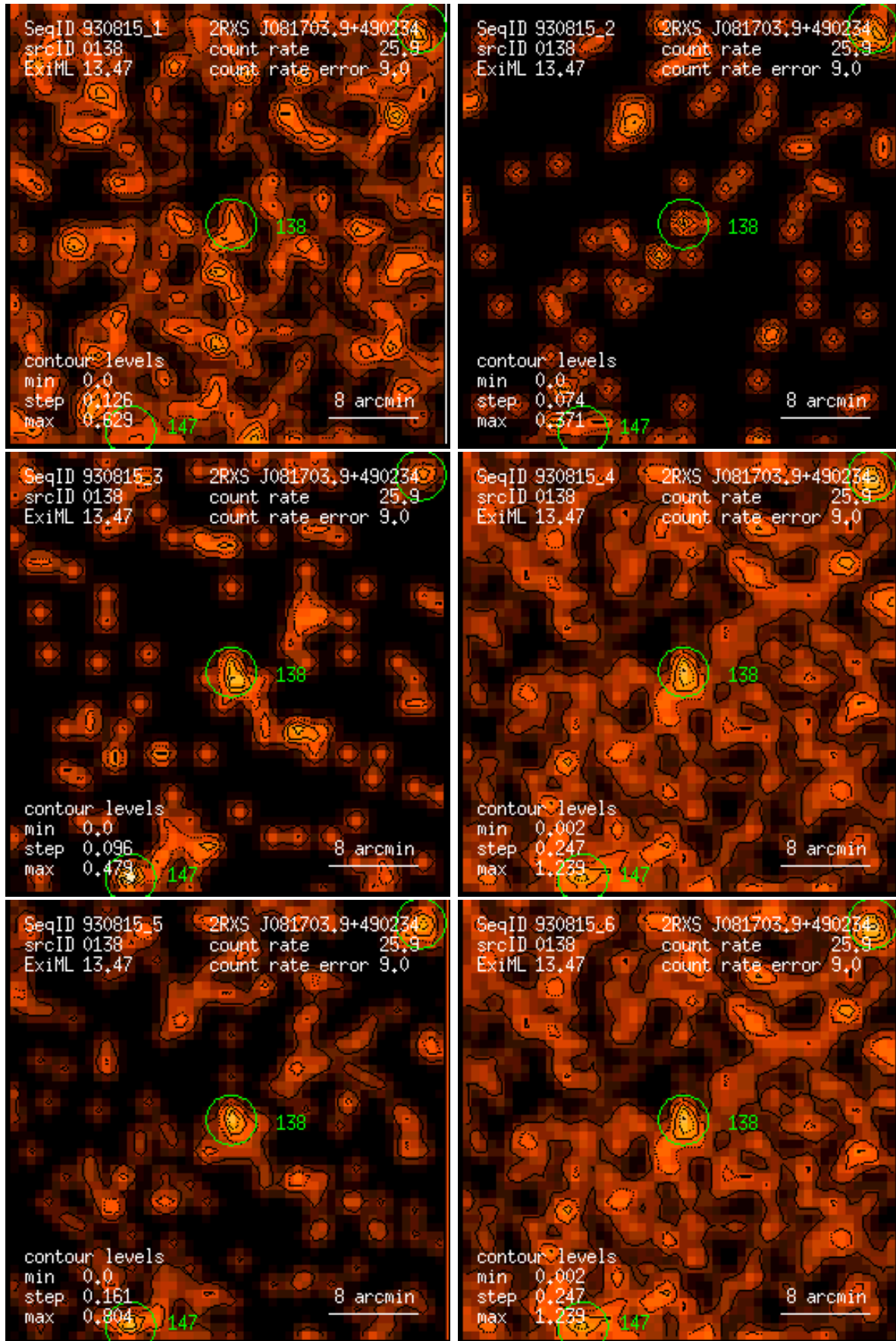
Figure 138: RASS 930815: detection 0138: band rate images, Gaussian filter: (1) PSPC channels 11 – 41, (2) 52 – 90, (3) 91 – 201, (4) 11 – 235, (5) 52 – 201, (6) 11 – 201. Broad band rates in counts/ks. Band rate contour levels in counts/ks/arcmin 2 .
