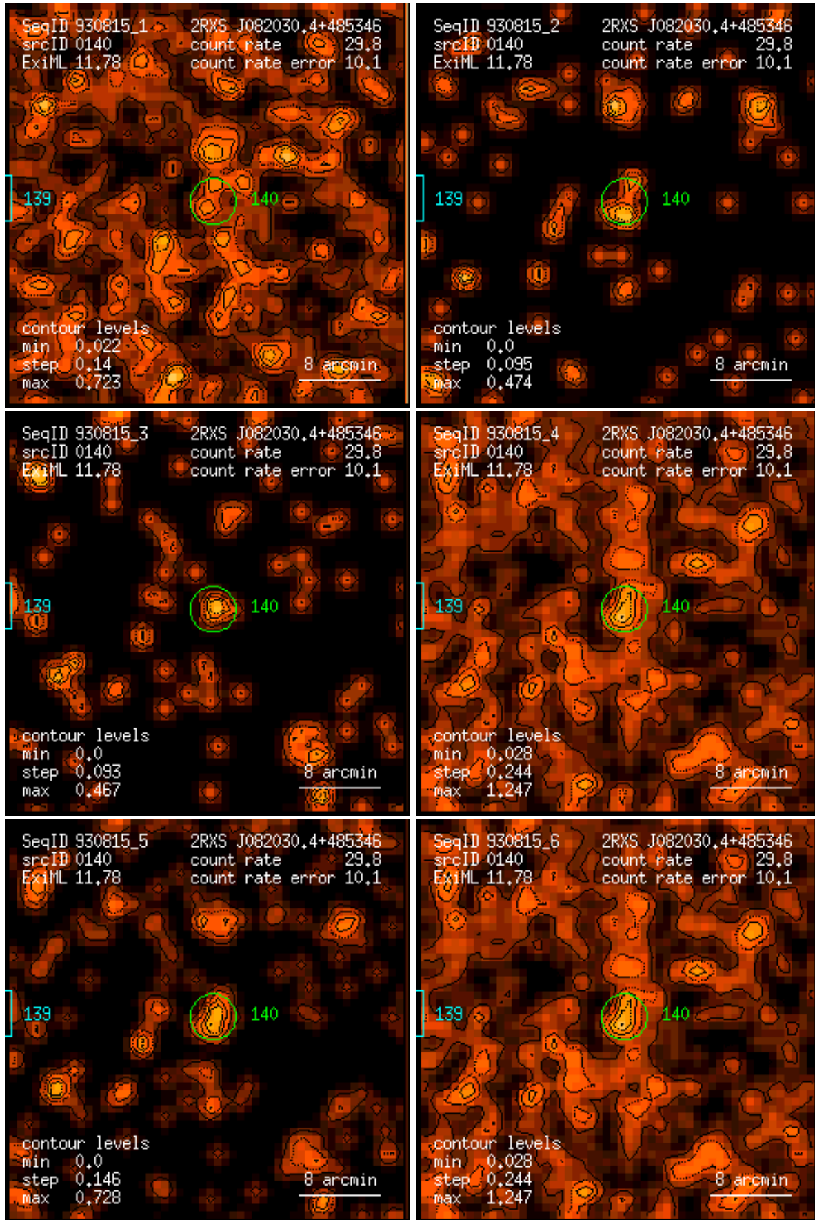
Figure 140: RASS 930815: detection 0140: band rate images, Gaussian filter: (1) PSPC channels 11 – 41, (2) 52 – 90, (3) 91 – 201, (4) 11 – 235, (5) 52 – 201, (6) 11 – 201. Broad band rates in counts/ks. Band rate contour levels in counts/ks/arcmin 2 .
