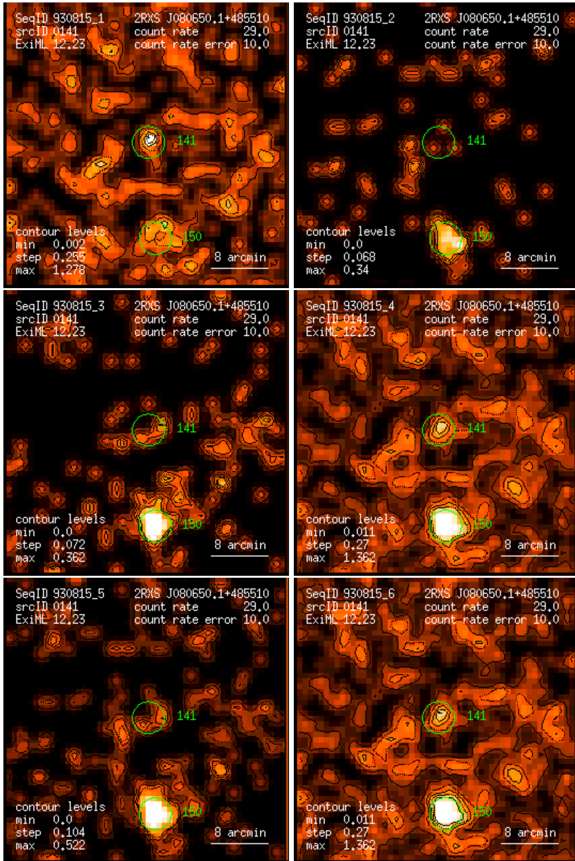
Figure 141: RASS 930815: detection 0141: band rate images, Gaussian filter: (1) PSPC channels 11 – 41, (2) 52 – 90, (3) 91 – 201, (4) 11 – 235, (5) 52 – 201, (6) 11 – 201. Broad band rates in counts/ks. Band rate contour levels in counts/ks/arcmin 2 .
