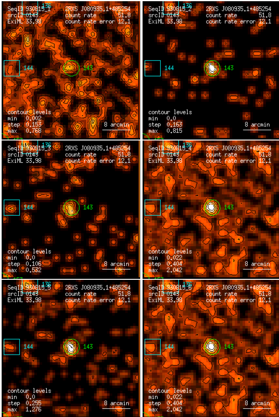
Figure 143: RASS 930815: detection 0143: band rate images, Gaussian filter: (1) PSPC channels 11 – 41, (2) 52 – 90, (3) 91 – 201, (4) 11 – 235, (5) 52 – 201, (6) 11 – 201. Broad band rates in counts/ks. Band rate contour levels in counts/ks/arcmin 2 .
