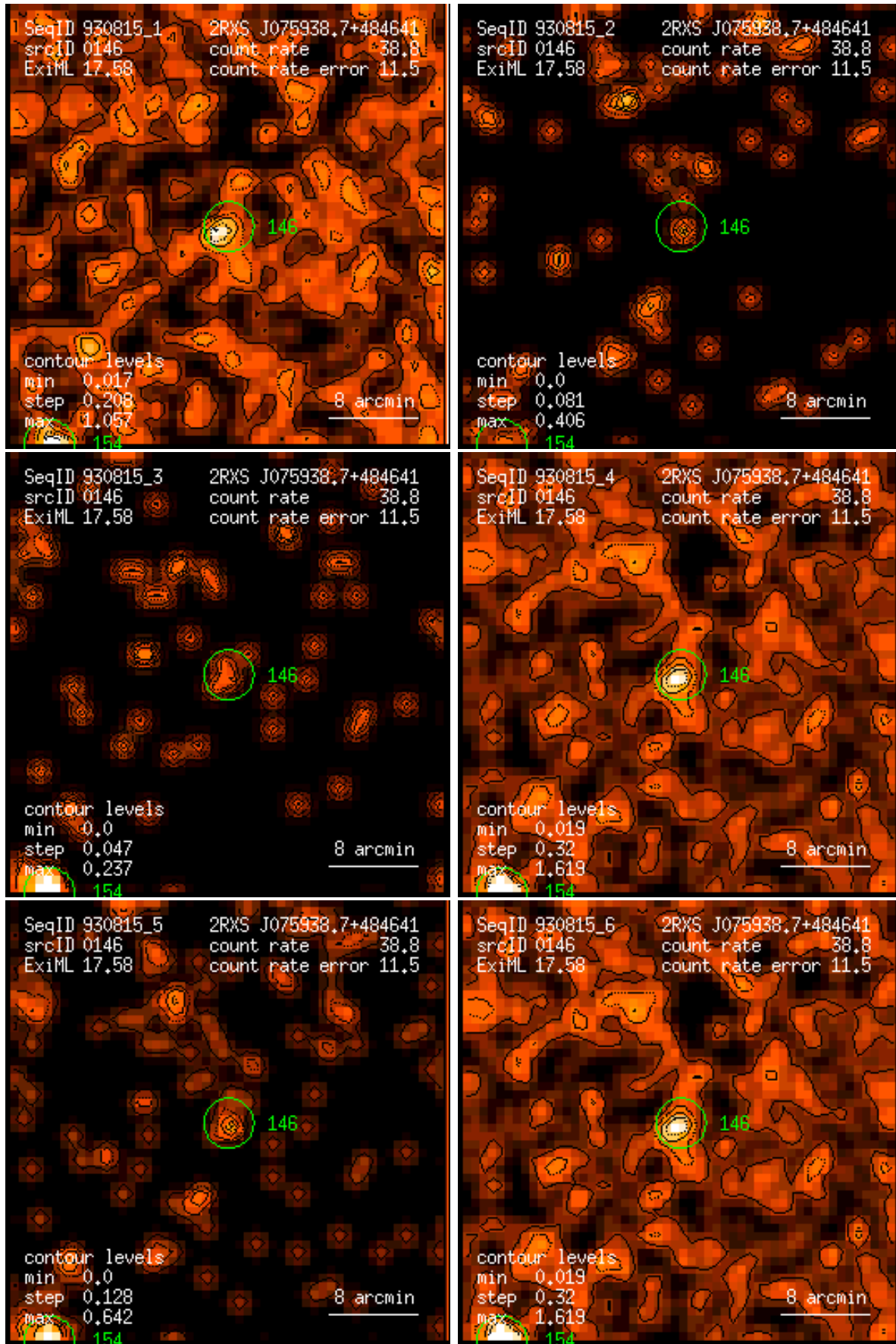
Figure 146: RASS 930815: detection 0146: band rate images, Gaussian filter: (1) PSPC channels 11 – 41, (2) 52 – 90, (3) 91 – 201, (4) 11 – 235, (5) 52 – 201, (6) 11 – 201. Broad band rates in counts/ks. Band rate contour levels in counts/ks/arcmin 2 .
