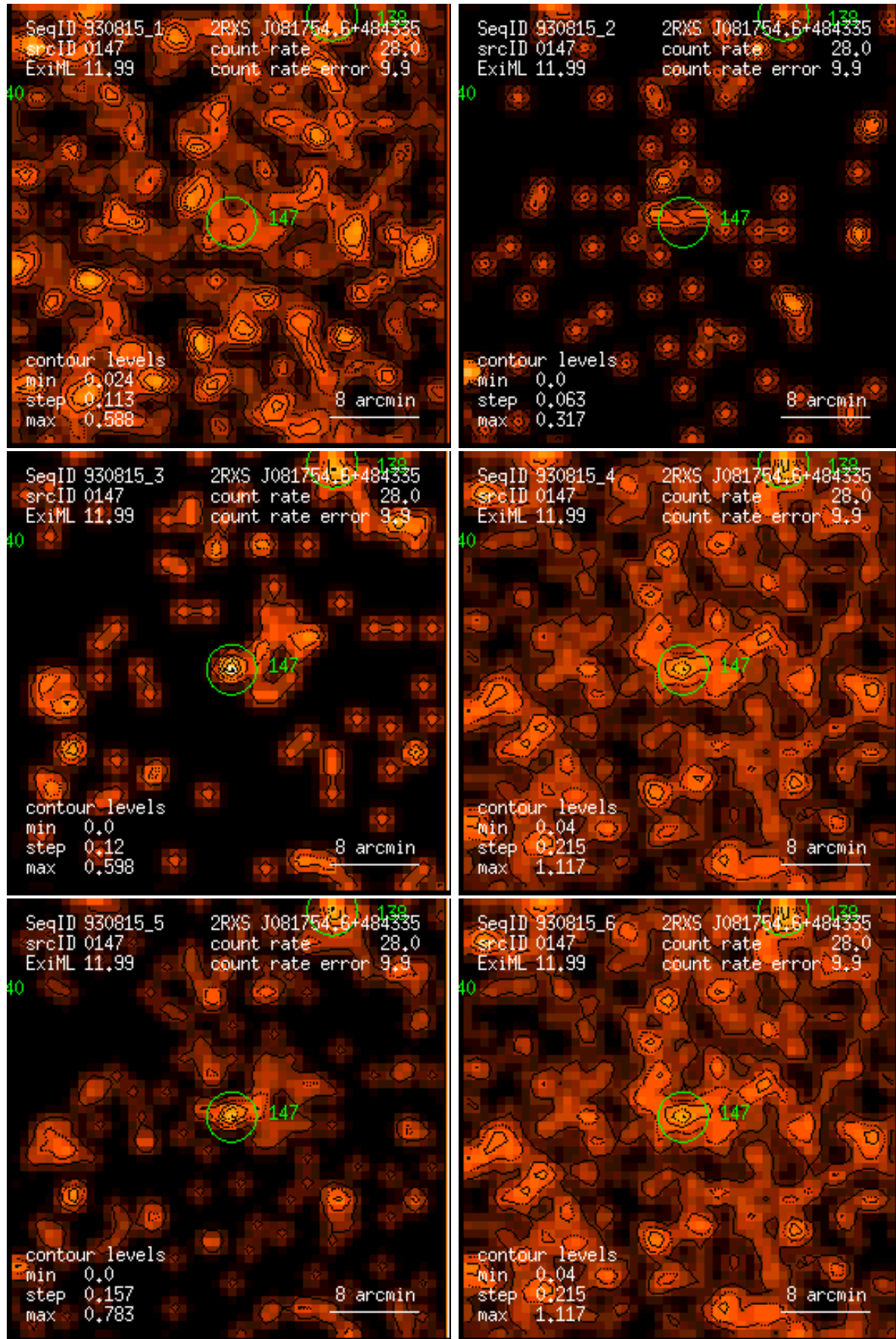
Figure 147: RASS 930815: detection 0147: band rate images, Gaussian filter: (1) PSPC channels 11 – 41, (2) 52 – 90, (3) 91 – 201, (4) 11 – 235, (5) 52 – 201, (6) 11 – 201. Broad band rates in counts/ks. Band rate contour levels in counts/ks/arcmin 2 .
