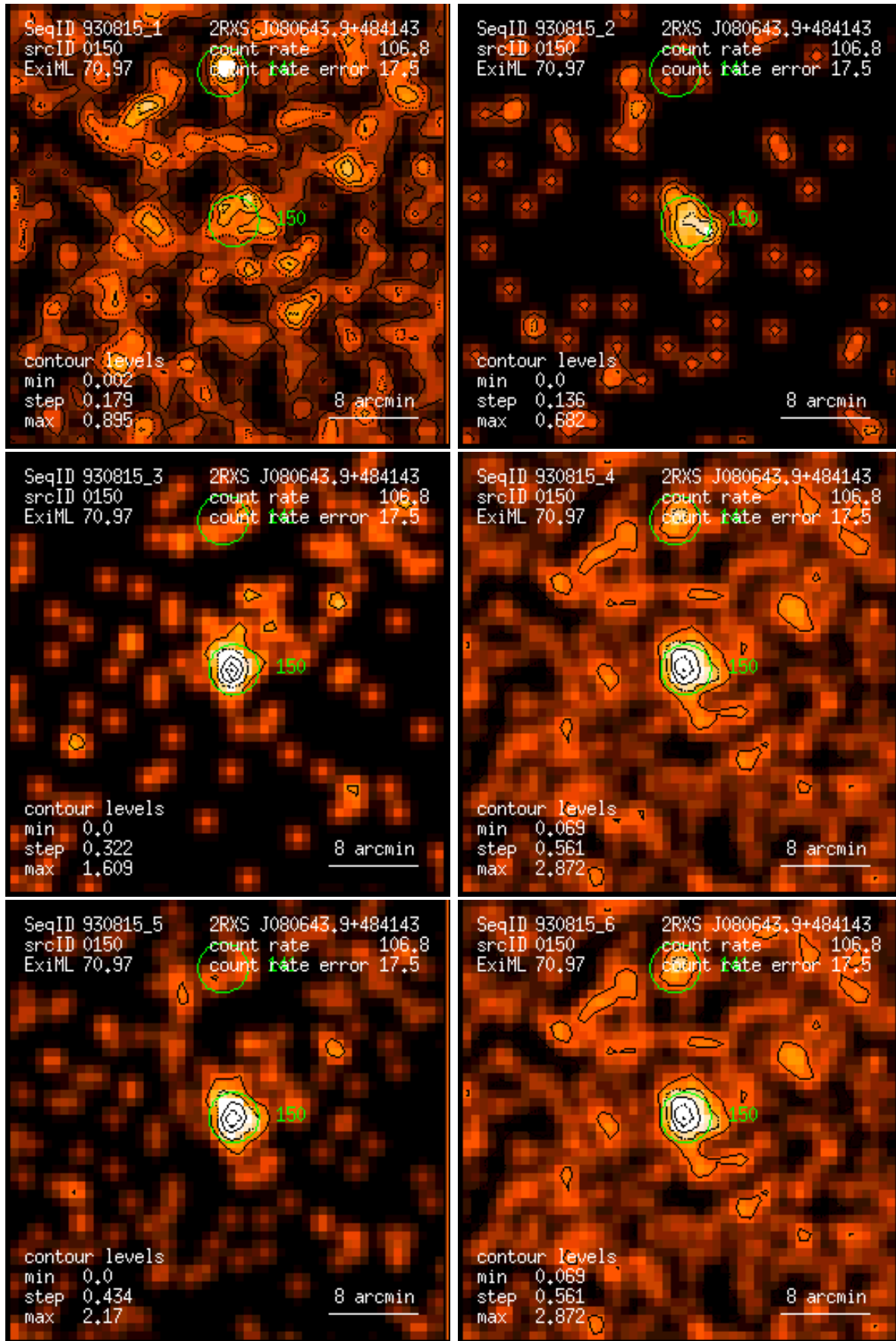
Figure 150: RASS 930815: detection 0150: band rate images, Gaussian filter: (1) PSPC channels 11 – 41, (2) 52 – 90, (3) 91 – 201, (4) 11 – 235, (5) 52 – 201, (6) 11 – 201. Broad band rates in counts/ks. Band rate contour levels in counts/ks/arcmin 2 .
